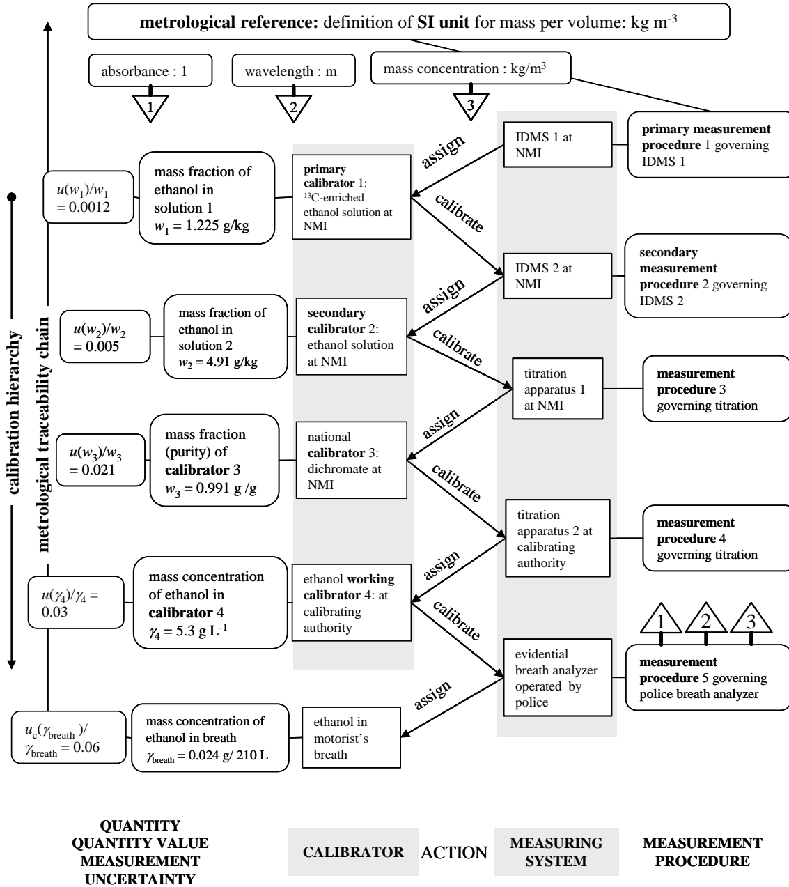
Figure 6: Traceability chain for measurements of breath alcohol with calibration via dichromate titration. IDMS = isotope dilution mass spectrometry. Adapted from [3].
