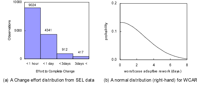
Fig. 1. An actual error correction effort histogram and a distribution for WCAR.
