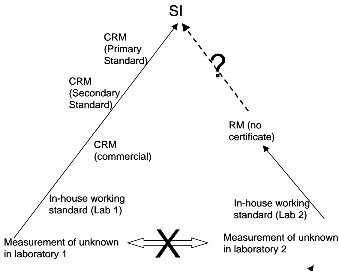
Figure 7: Without a traceable calibrator measurement results obtained in different laboratories cannot be comparable.
