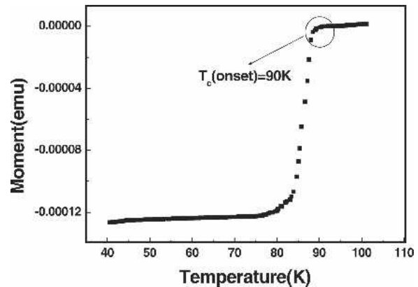
FIG. 8. Temperature dependence of magnetic moment for YBCO/YBiO 3 /LaAlO 3 yielding an onset critical temperature 90 K.
