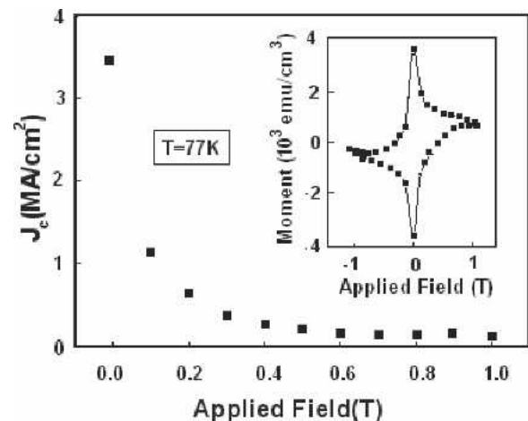
FIG. 9. Field dependence of critical current density at 77 K and self-field for YBCO films deposited on YBiO 3 buffered LaAlO 3 . Inset: Hysteresis loop of magnetization at 77 K.
