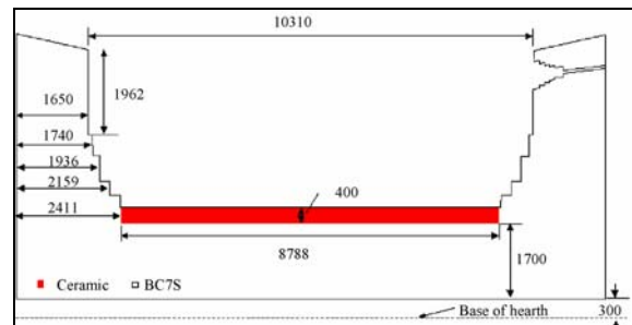
Figure 2: Geometric dimensions of PKBF5 hearth
