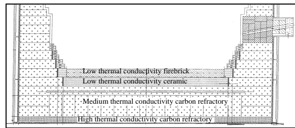
Figure 1: Port Kembla Blast Furnace 5 (PKBF5) hearth showing one taphole (right side) and different refractory materials at the start of its campaign
