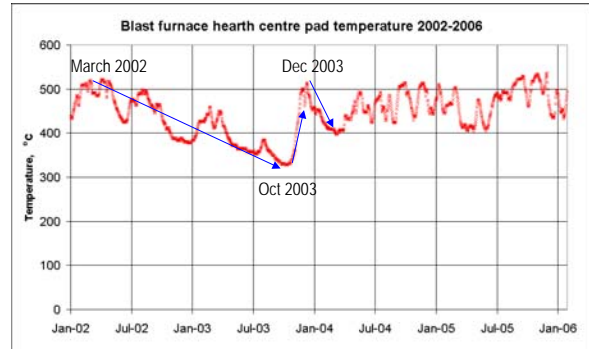
Figure 5: Centre pad temperature data for PKBF5 for January 2002 onwards
