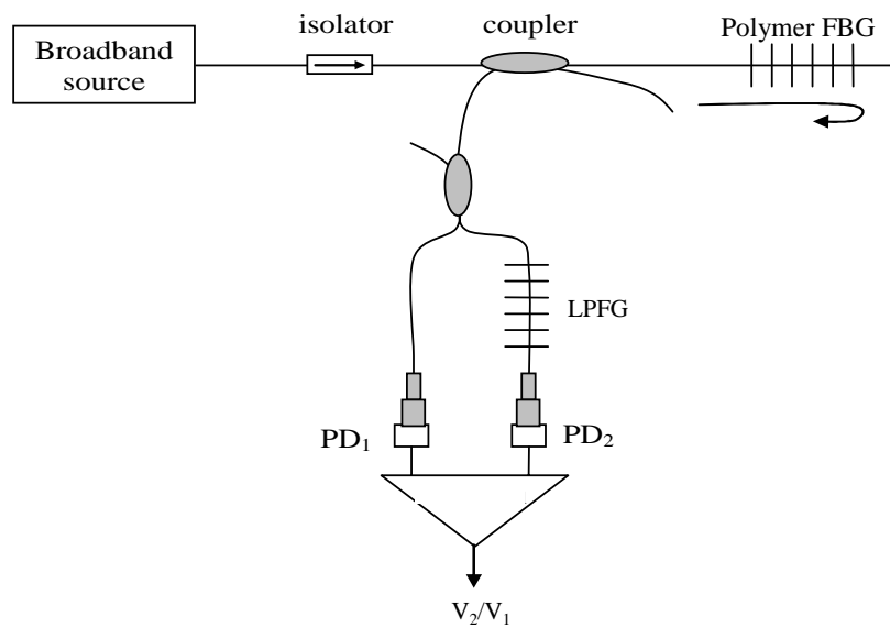
Fig. 2 Scheme of strain sensing using polymer fiber Bragg grating and long period fibre grating.
