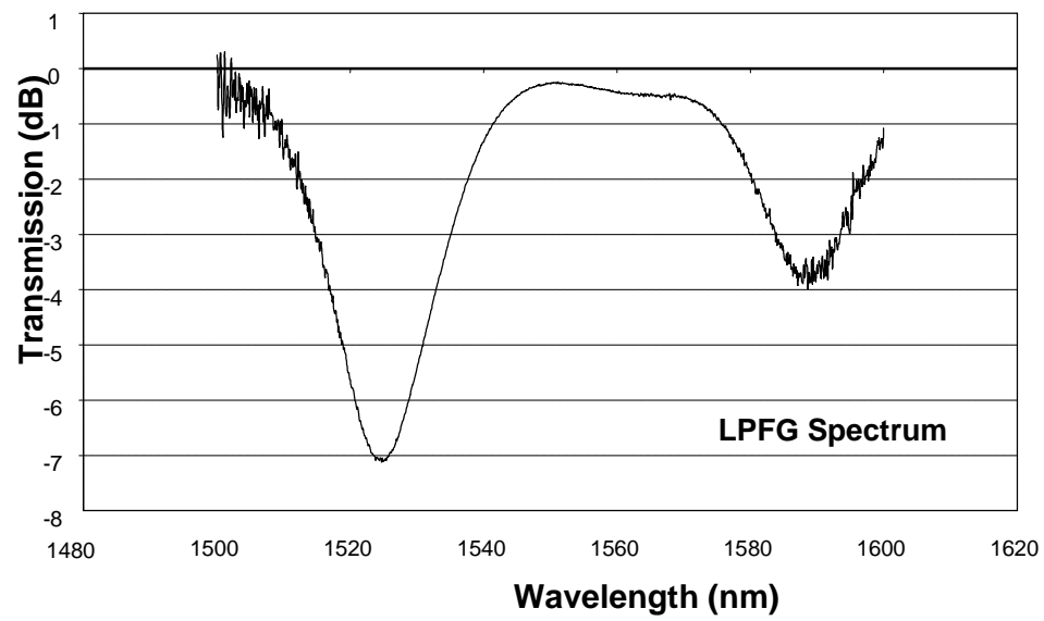
Fig. 1 Spectrum of the long period fibre gratings
