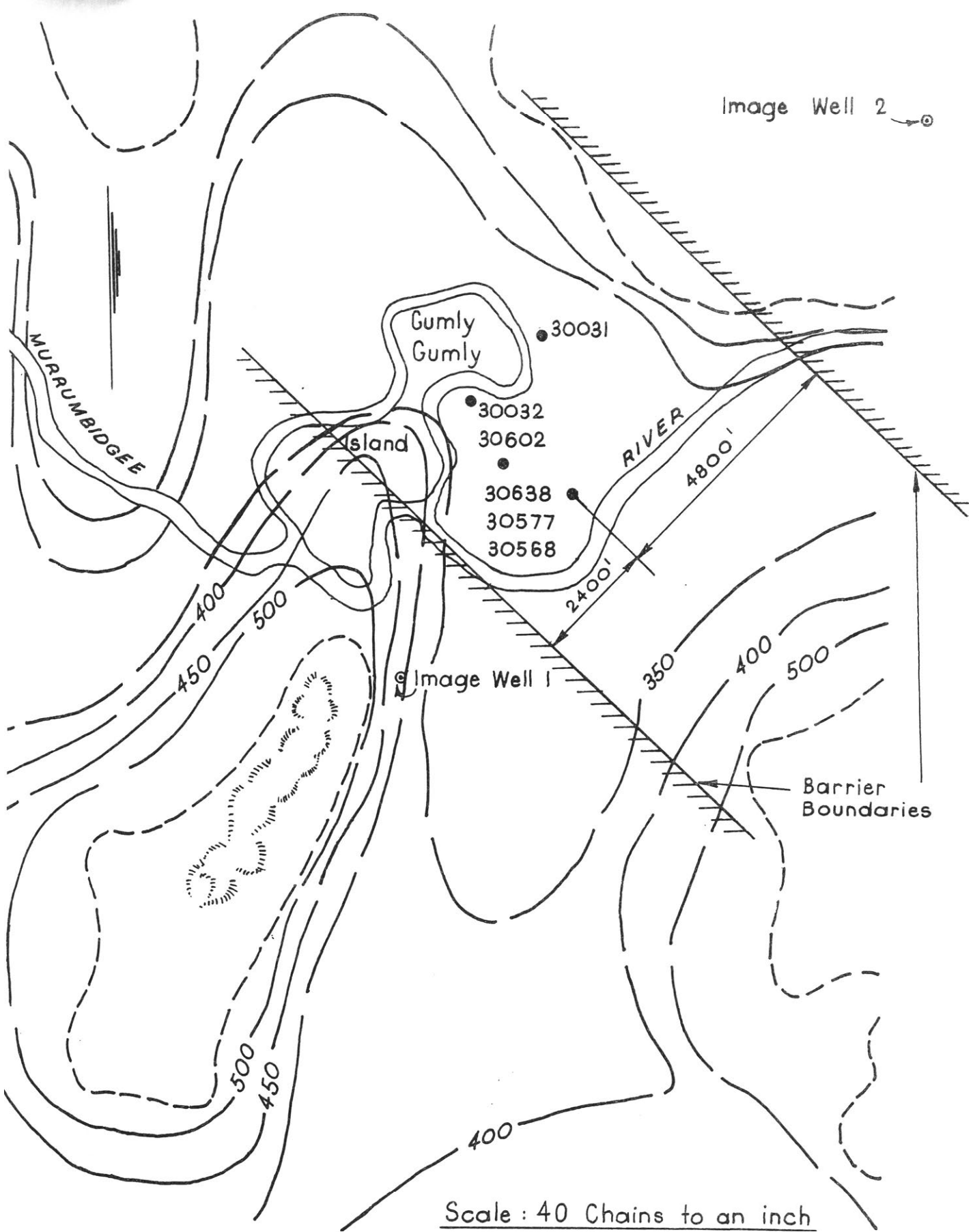
Fig. 2.8: Location and direction of Barrier Boundaries.
