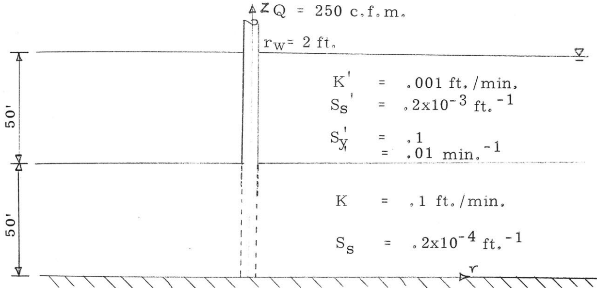
Fig. 3.16: Flow system for test problem.
