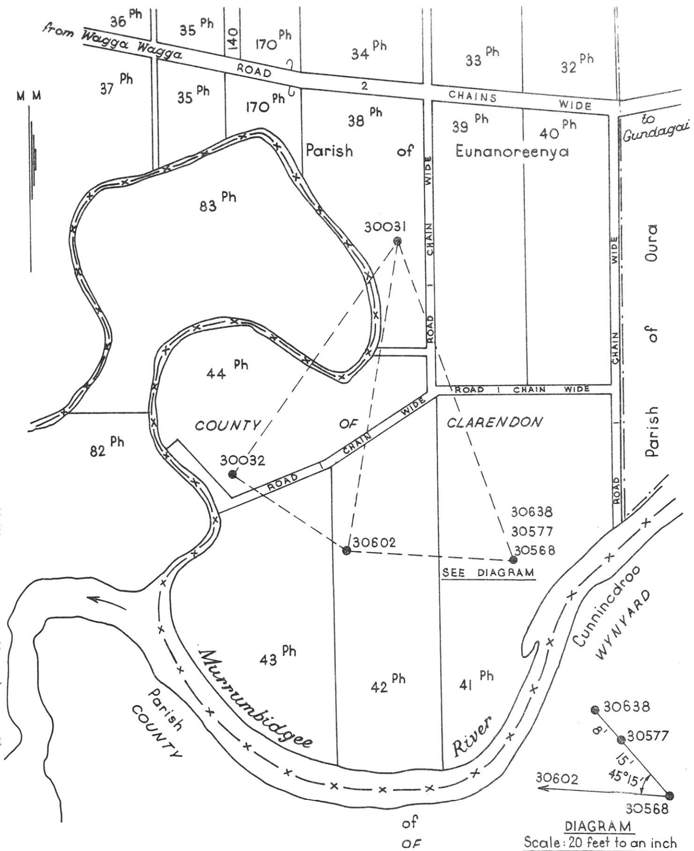
Fig. 2.1: General Plan of Site A.
