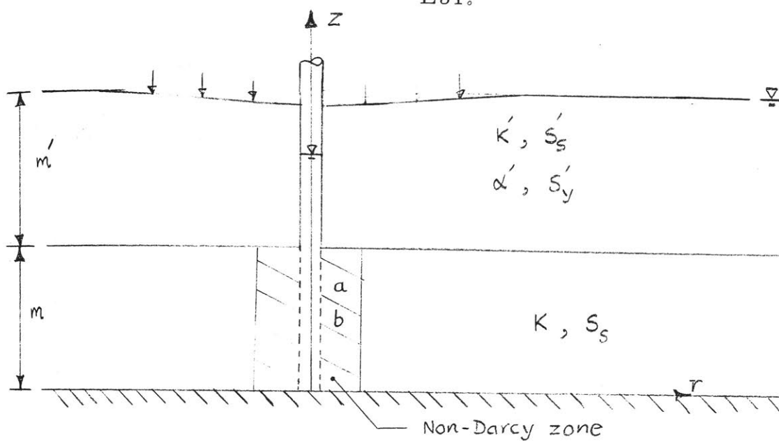
Fig. 3.15: Mathematical model for Rosevale well-aquifer system.
