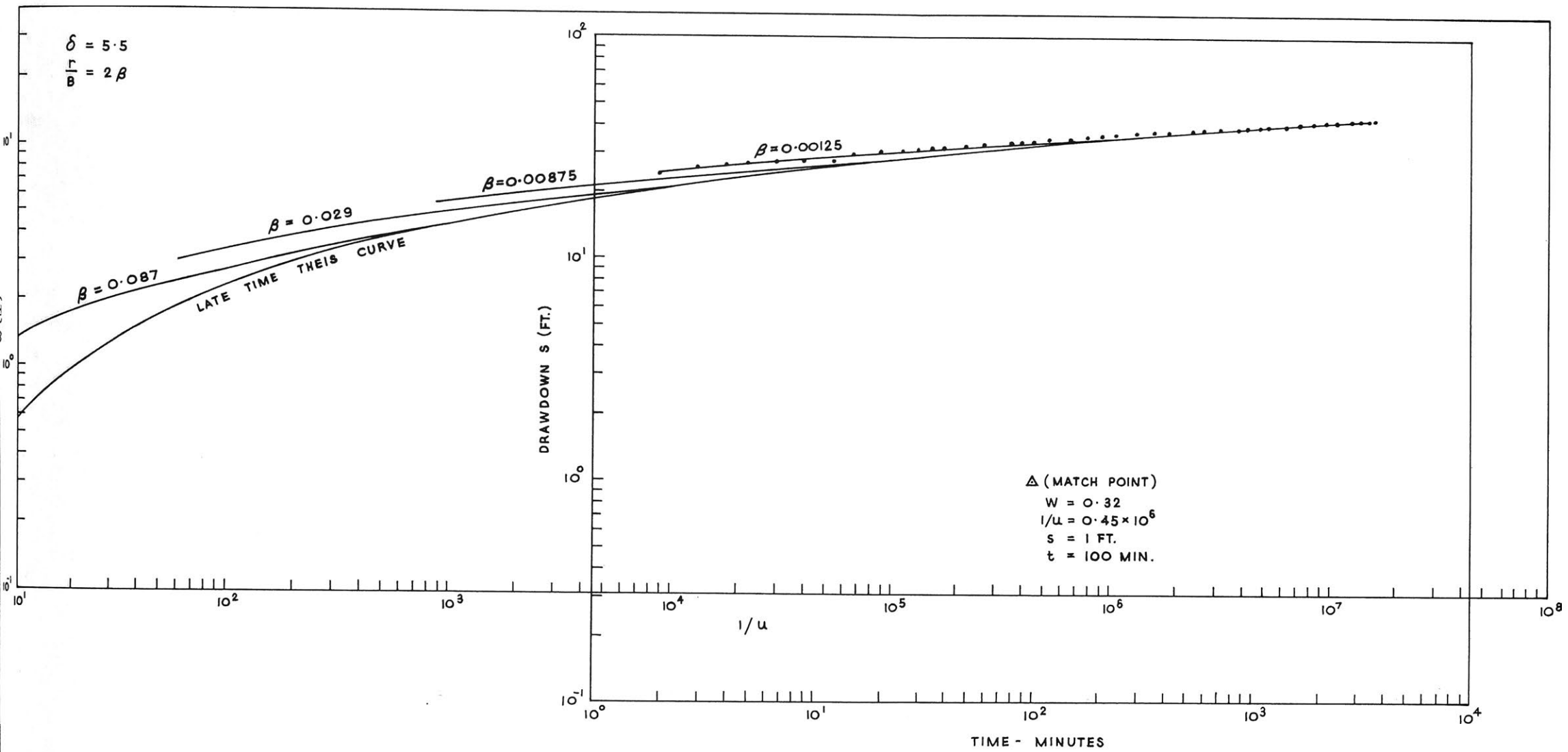
Fig. 2.30: Matching of Field Data on Type Curves for Main Aquifer.
