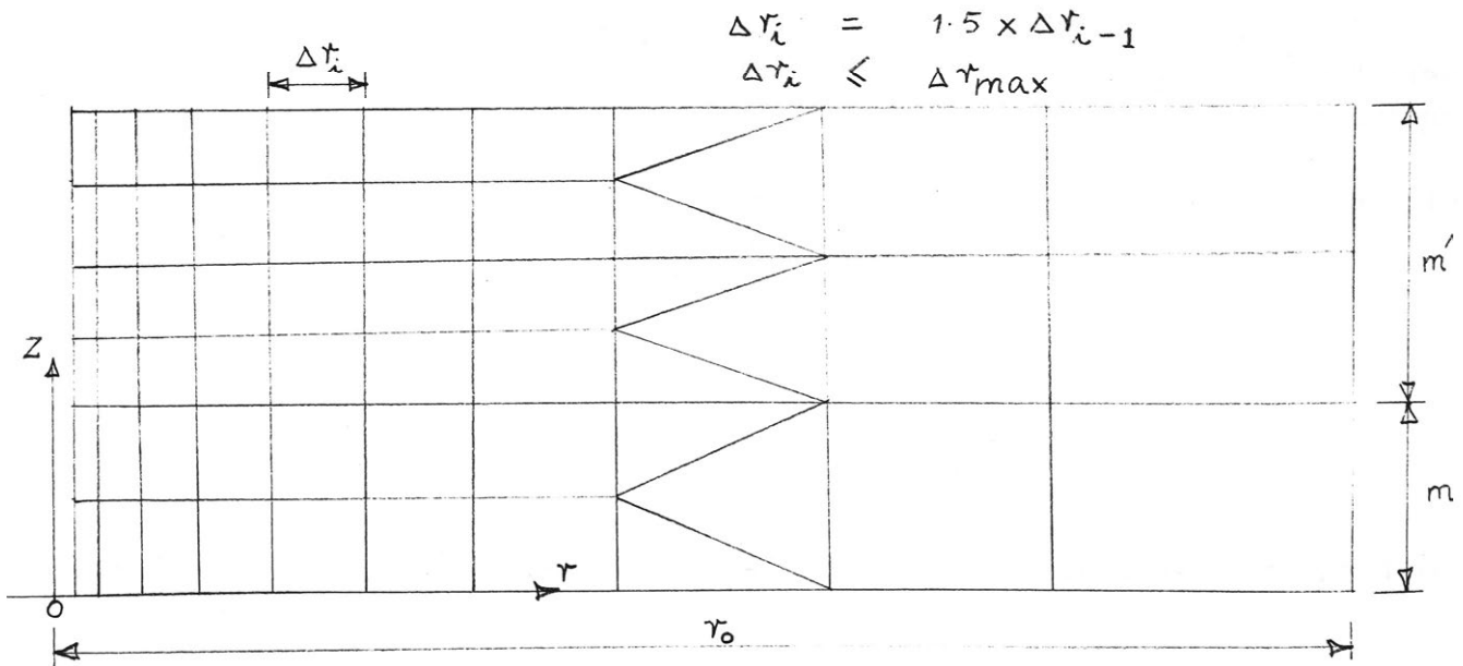
Fig. 2.21: Typical two-dimensional finite element network.
