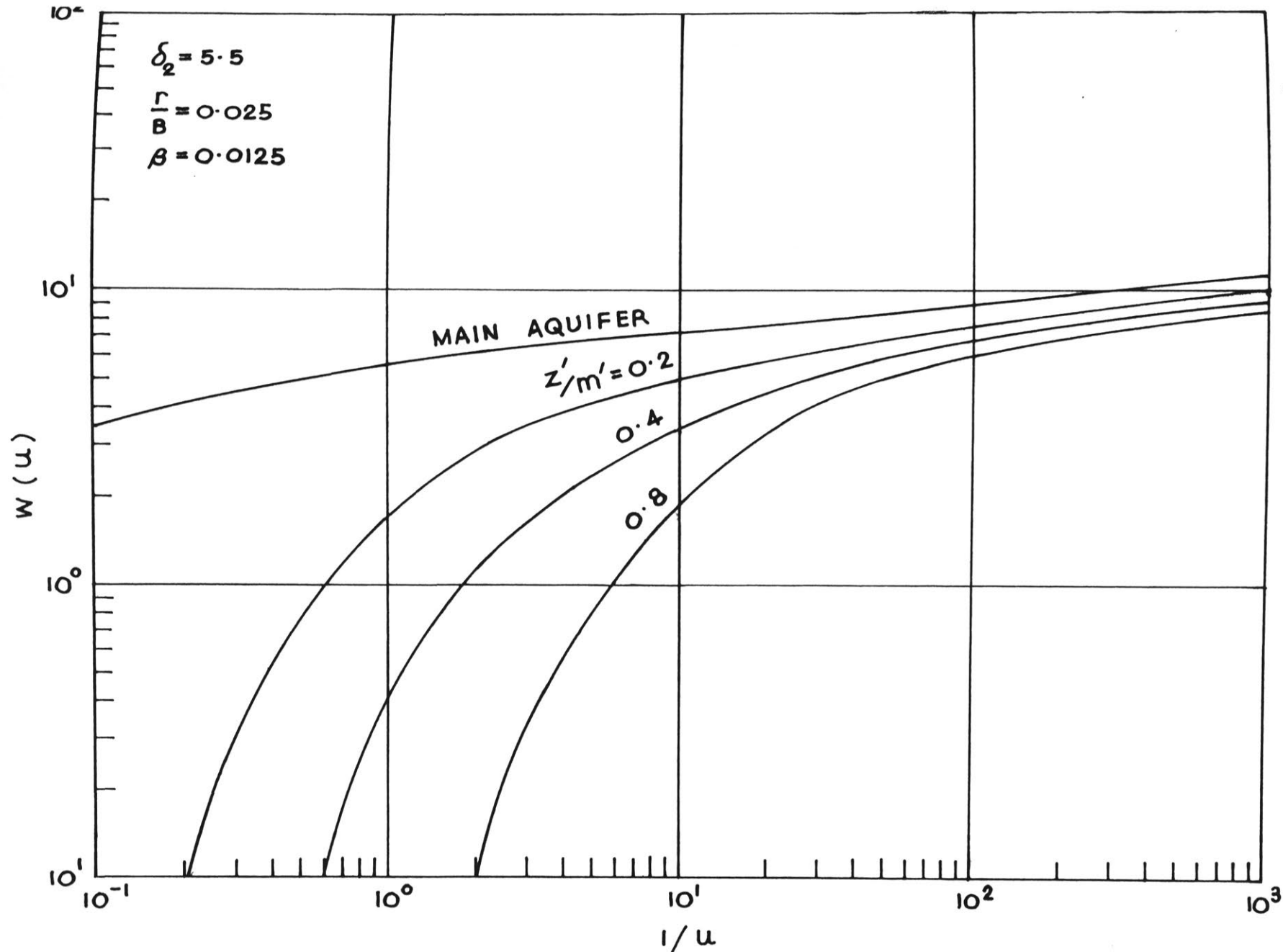
Fig. 2.29: Type curves for the overlying aquitard of a confined aquifer-aquitard system.
