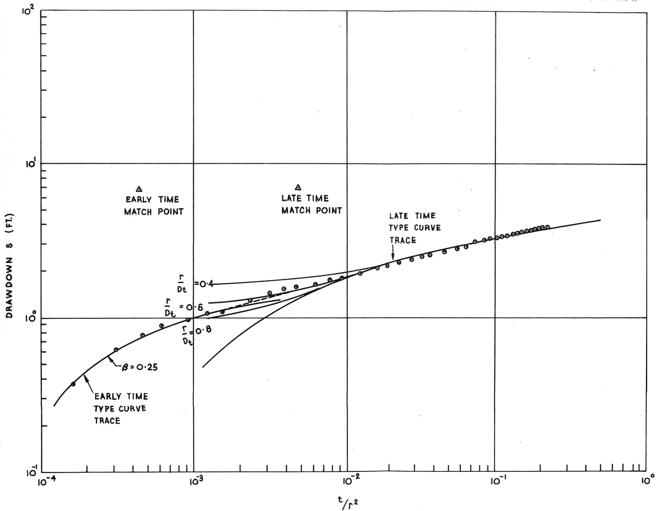
Fig. 3.8: Time-Drawdown Graph for Observation Well 14S9A - Test 1.
