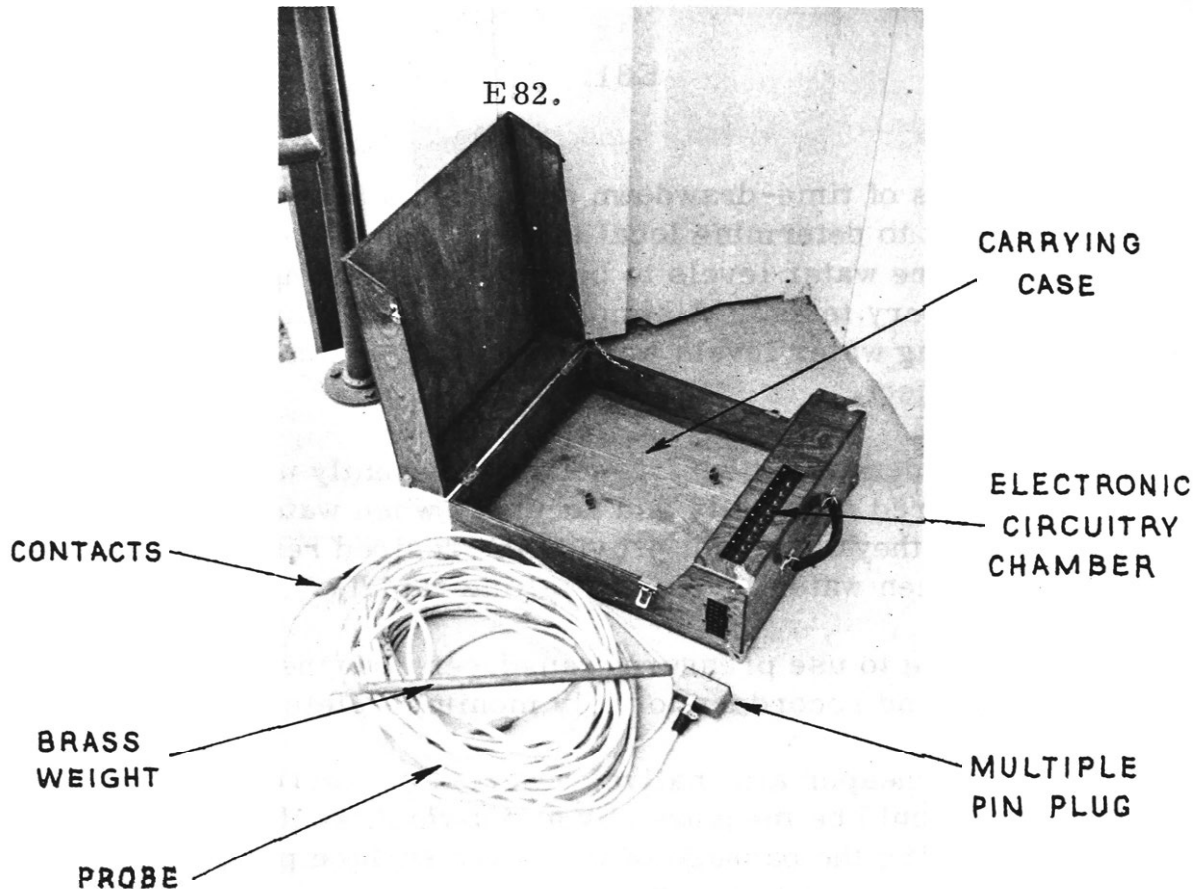
Fig. III-1 Multiple Contact Electric Probe.
