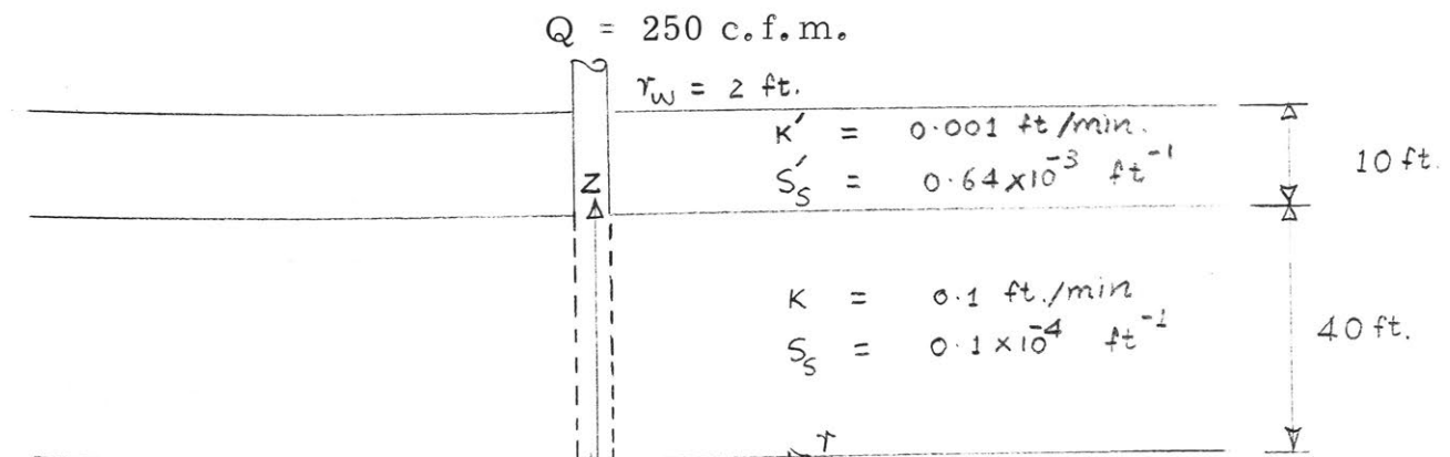
Fig. 2.22: Flow System for Test Problem
