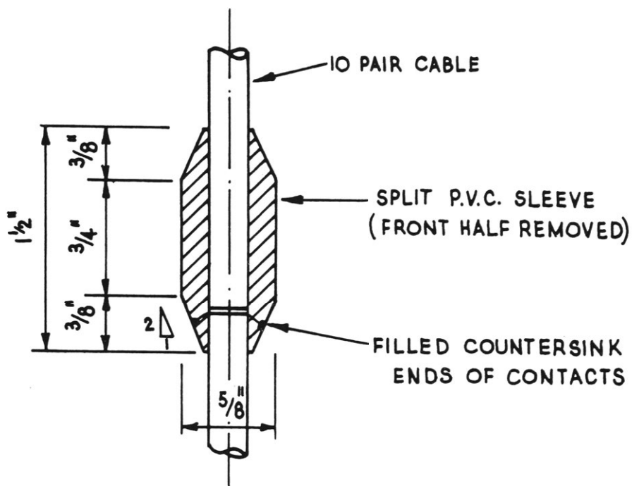
Fig. III-3: Detail of P.V.C. Sleeves
