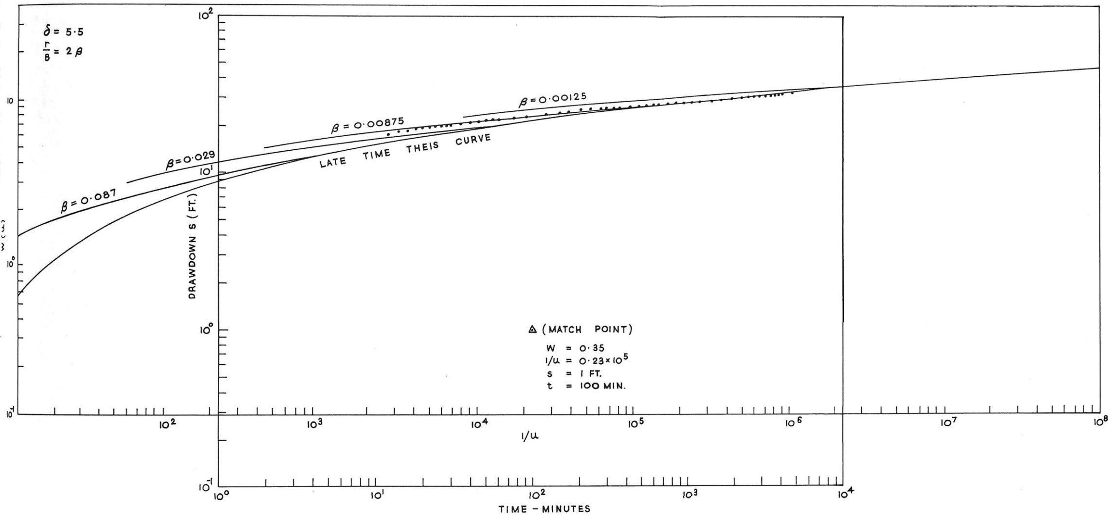
Fig. 2.31: Matching of Field Data on Type Curves for Main Aquifer.
