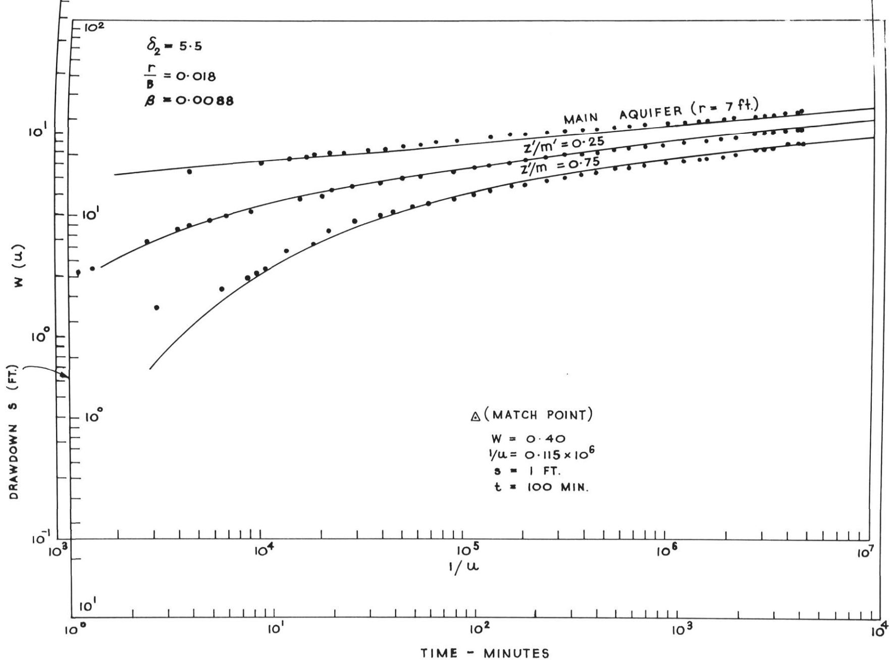
Fig. 2.32: Matching of Field Data on Type Curves for Aquifer-Aquitard System.
