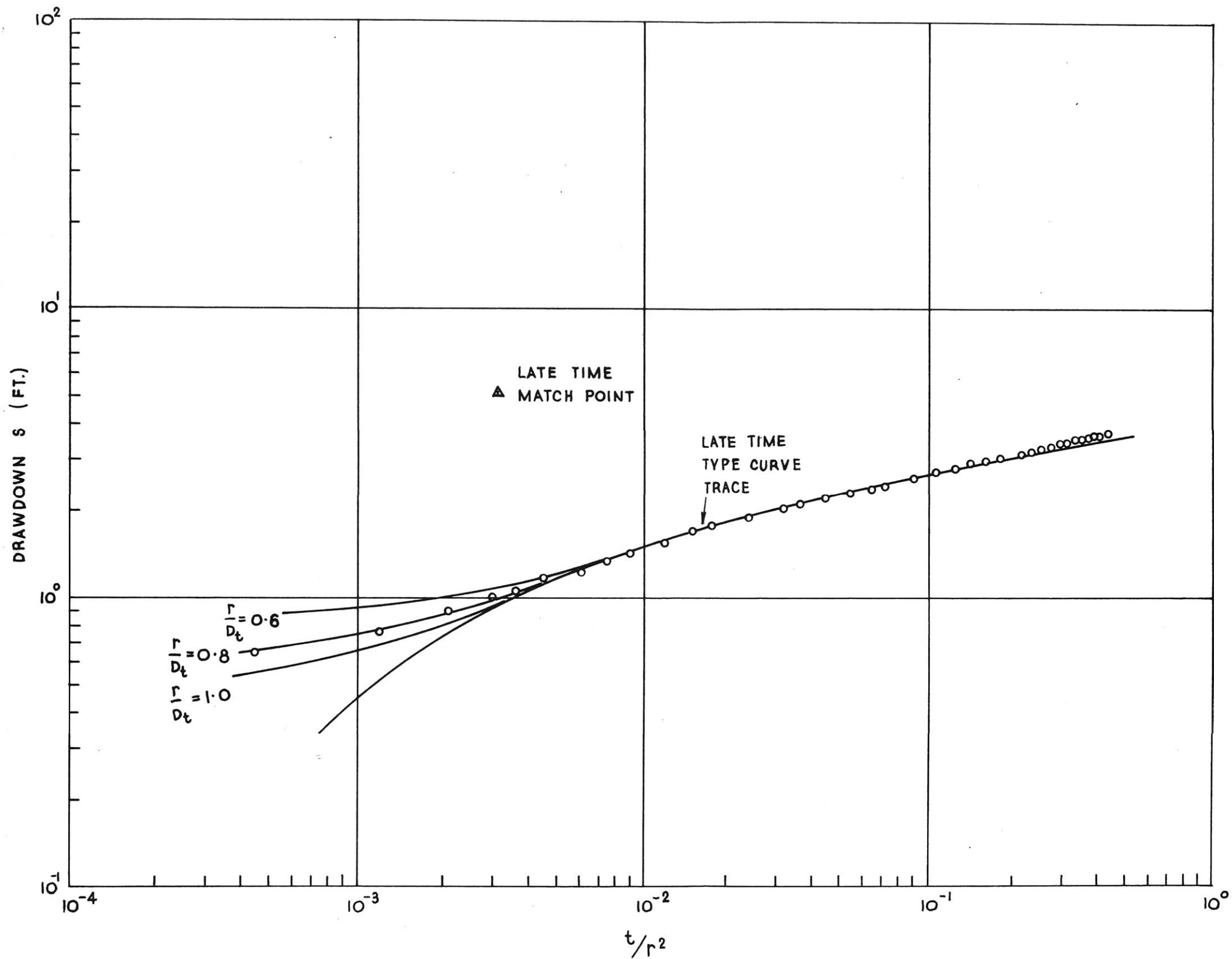
Fig. 3.7: Time-Drawdown graph for observation well 4 - Test 1.
