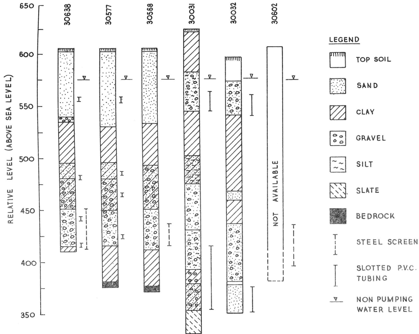
Fig. 2.2 Construction features and available drillers logs of wells at Site A.
