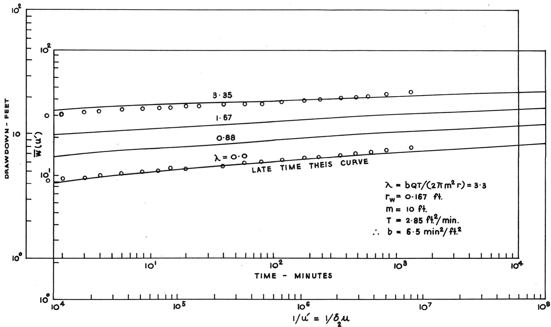
Fig. 3.23: Matching of field data on non-Darcy flow type curves.
