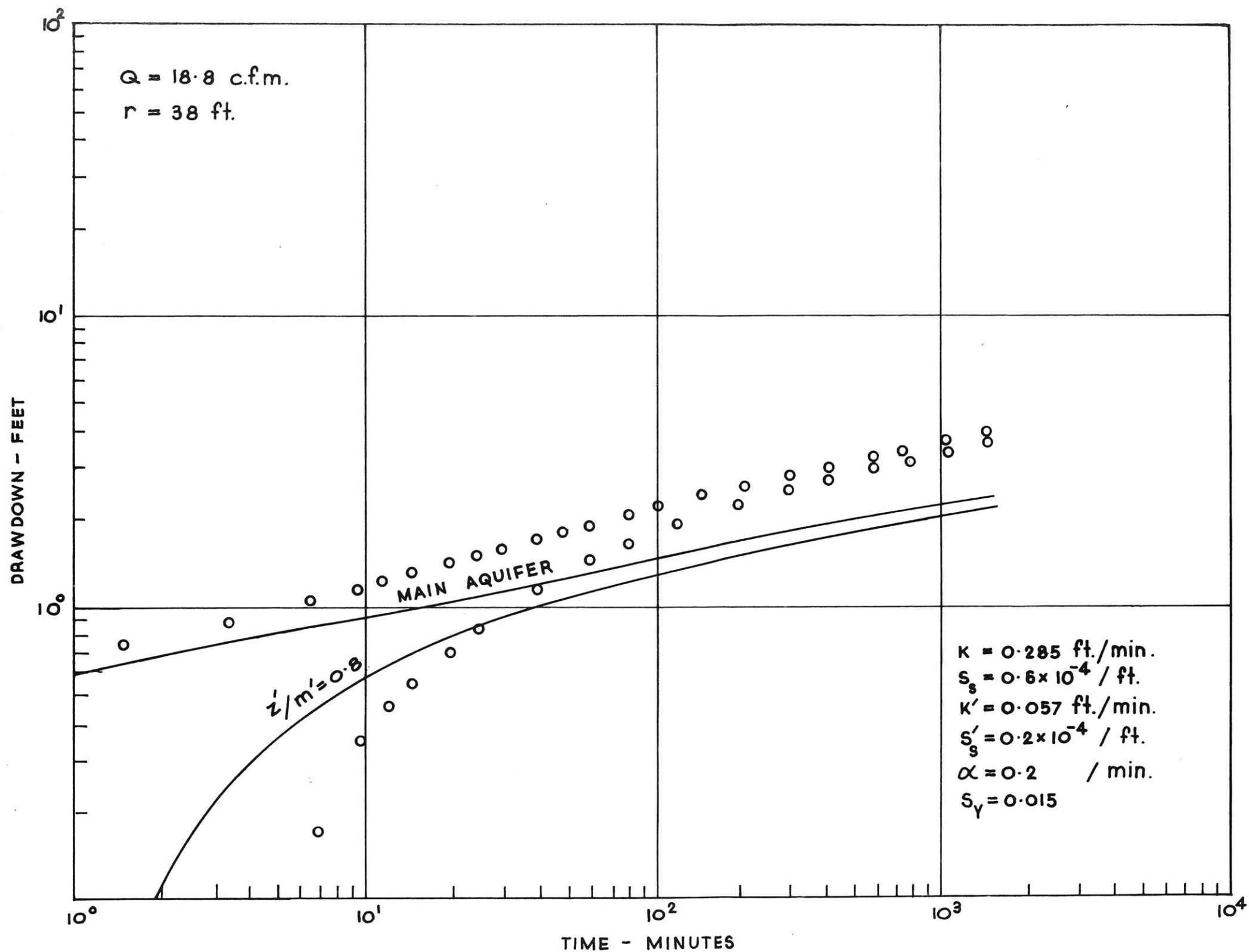
Fig. 3.25: Comparison of finite element model results with field data.
