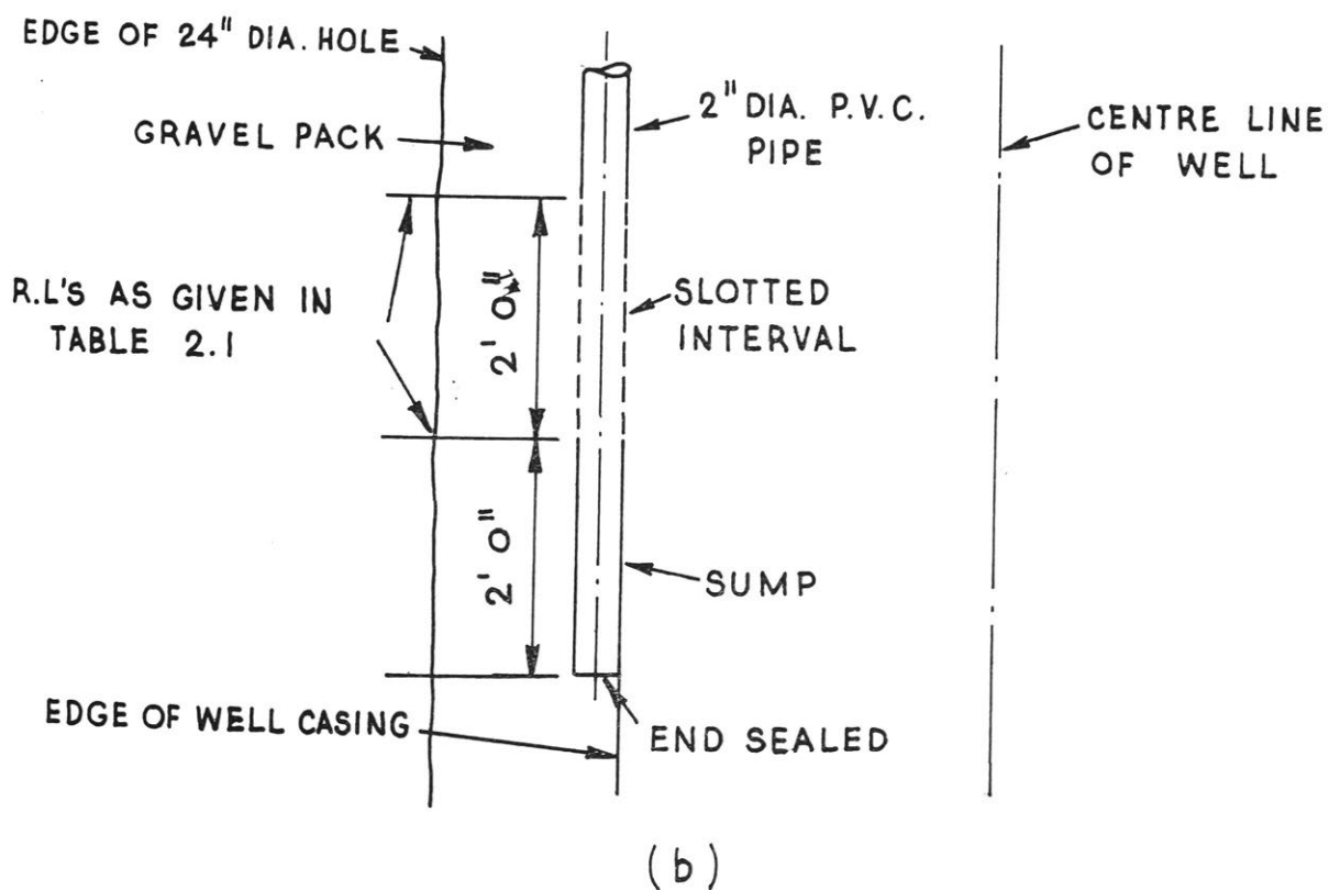
Fig. 2.4: Positioning and details of slotted P.V.C. piezometers in production well 30638.
