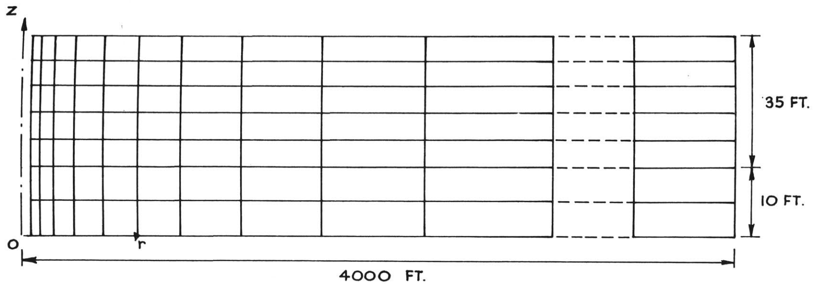
(a) COARSE MESH (NO. OF NODES = 184)
