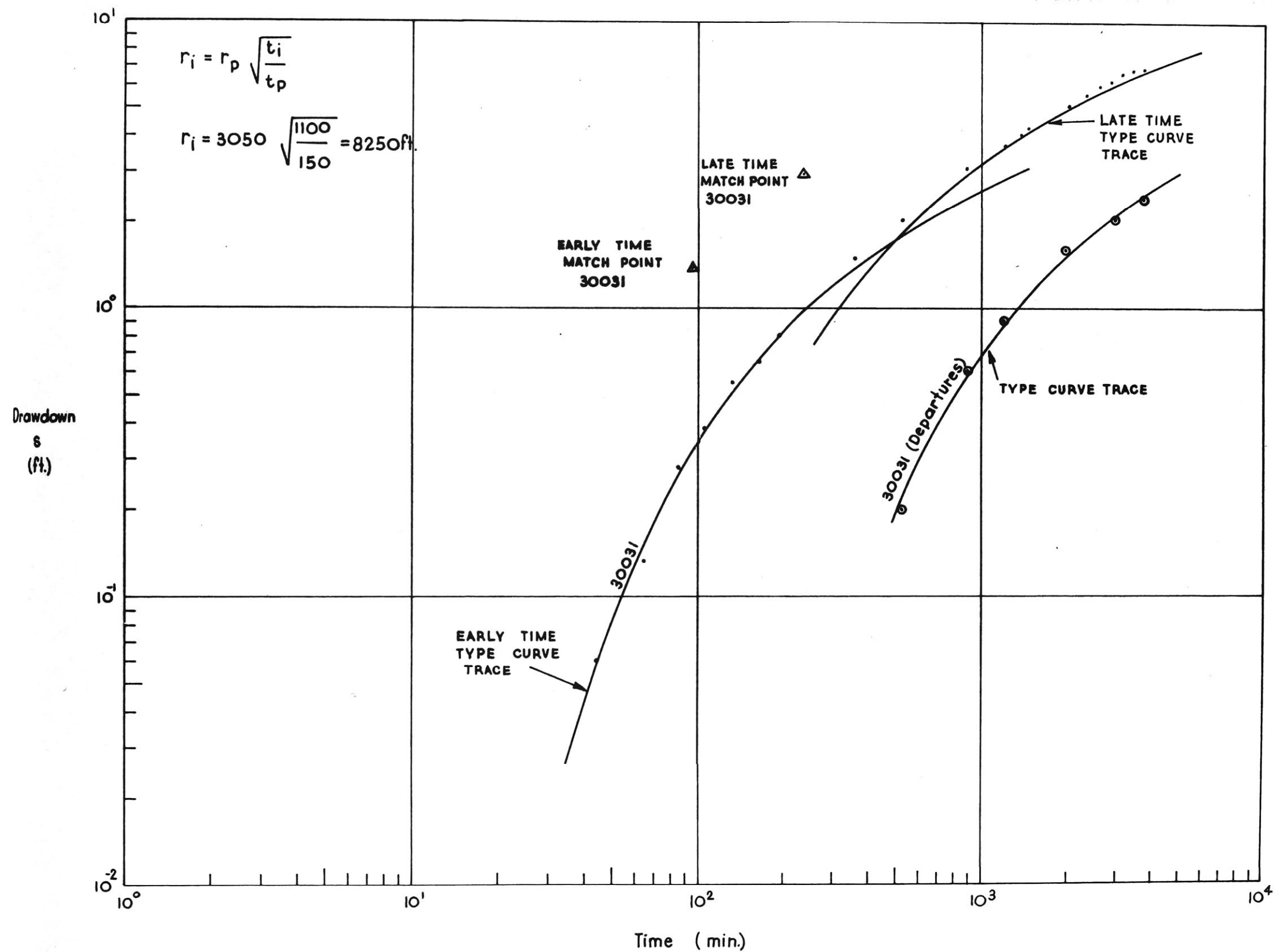
Fig. 2.7: Time Drawdown Graph of Observation Well 30031.
