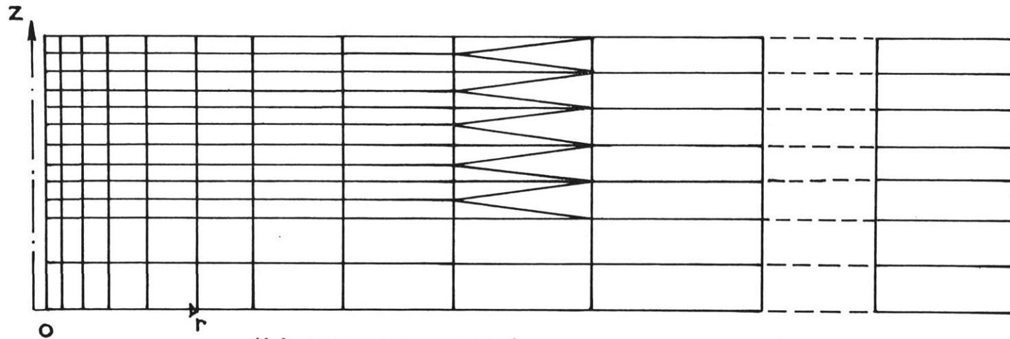
(b) REFINED MESH (NO. OF NODES = 229)
