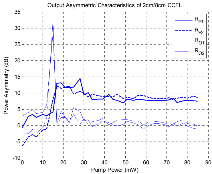
Figure 10. Output power ratios of the 2cm/8cm CCFL.
