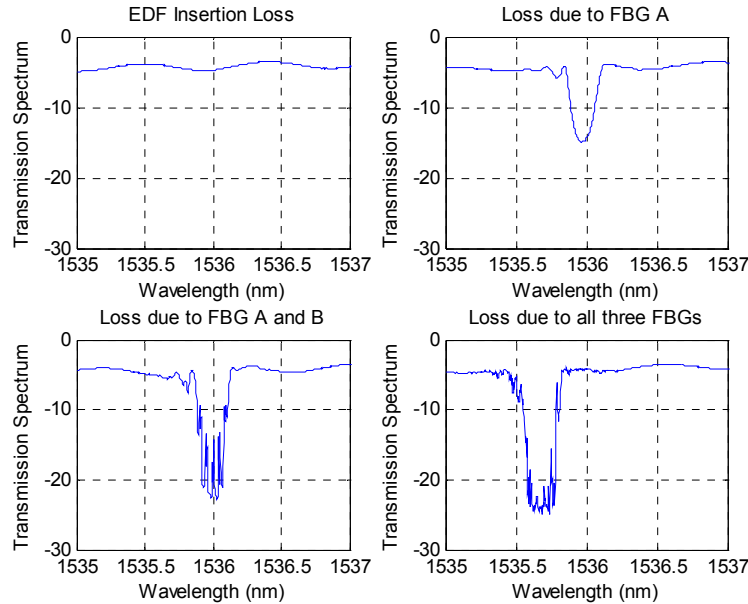
Figure 3. Transmission spectra of a 2cm/8cm CCFL obtained with a tunable laser, at various stages of fabrication.
