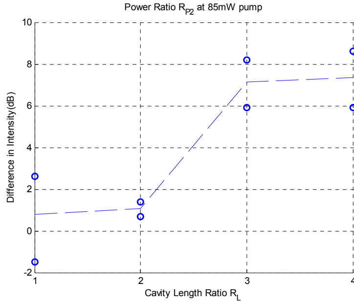
Figure 11. Power asymmetry R_{p2} of various CCFLs when pumped at 85mW. Dashed line obtained by averaging measurements.
