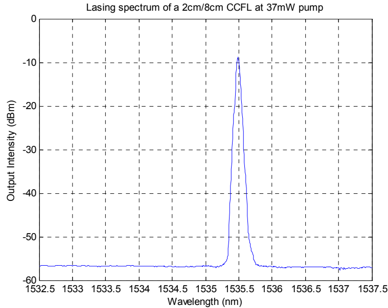
Figure 5. Lasing spectrum at 37mW pump power recorded with OSA, under the P_{21} arrangement. Sensitivity was set to -70dBm.
