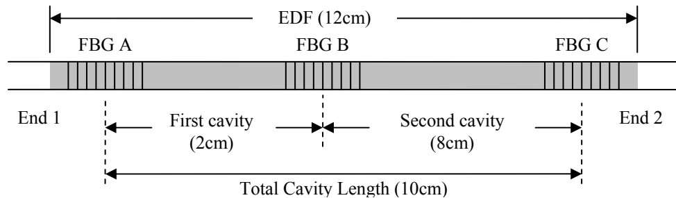
Figure 2. Schematic of the 2cm/8cm CCFL.
