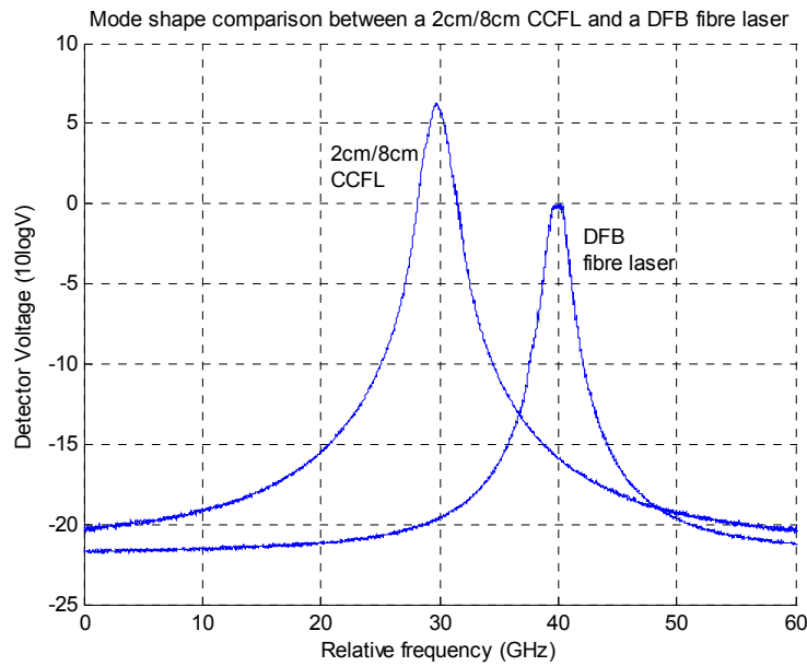
Figure 6. Lasing mode shapes of the 8cm/2cm CCFL (under P_{22} ) and a DFB fibre laser.
