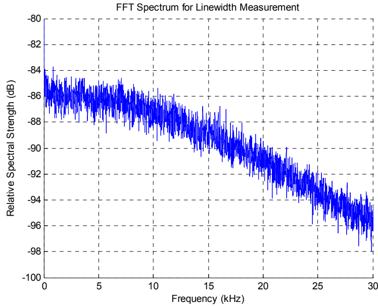
Figure 7. Linewidth measurement of a 2cm/8cm CCFL using delayed self-homodyne technique.
