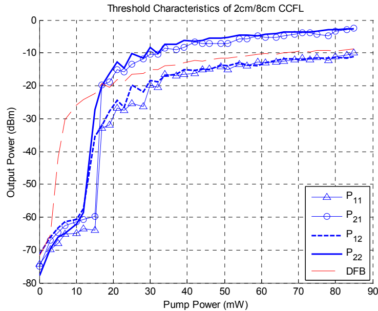
Figure 8. Threshold characteristics of all four pump-output arrangements of a 2cm/8cm CCFL, and threshold characteristic of a DFB fibre laser for comparison.
