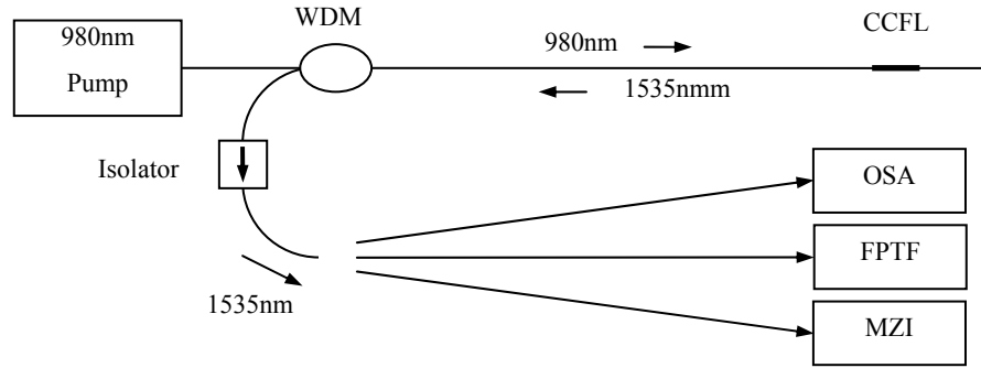
Figure 4. Schematic of testing system.
