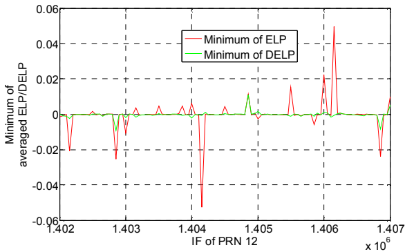
Figure 14 – Comparison of minimum values of averaged ELP with that of DELP for PRN 12 in the presence of PRN 25 (IF=1405150 Hz) and multipath in PRN 25 signal with relative amplitude of 0.3 and phase difference of 1.9672\pi
