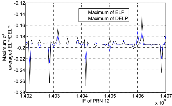
Figure 9 – Comparison of maximum values of averaged ELP with that of DELP for PRN 12 in the presence of PRN 25 (IF=1405150 Hz) and multipath in PRN 12 signal with relative amplitude of 0.3 and phase difference of 0.4918\pi
