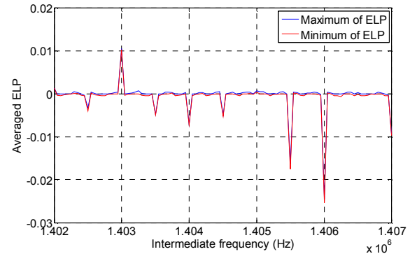
Figure 1 – ELP averaged over 20 msec in absence of multipath (PRN 12) [2]
