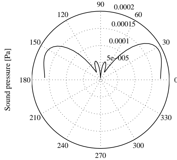
Figure 13: Directivity pattern at the second n=0 natural frequency of 44.5 Hz.
