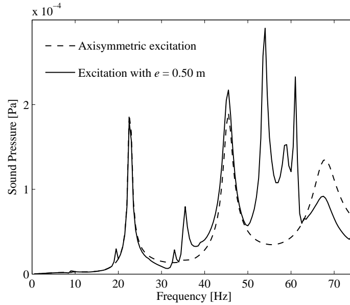
Figure 11: Maximum far field sound pressure, \theta = 0 , r = 1000 m.
