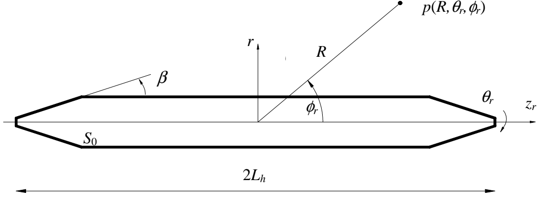
Figure 6: Coordinate system for the far field point.
