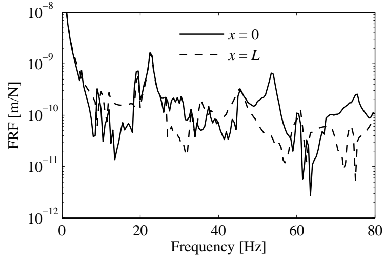
Figure 8: FRF of the axial displacement (force and moment excitation with e = 0.5 m).
