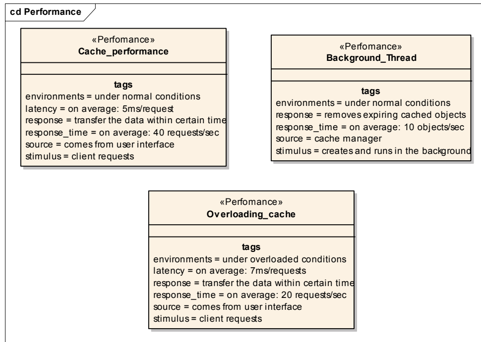
Figure 7. Performance NFRs
