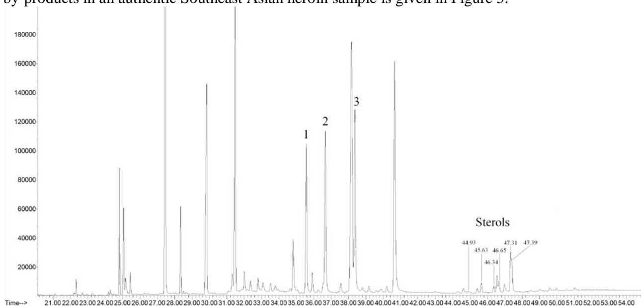
FIG. 5- Total ion current chromatogram of the acid/neutral extract of a typical SEA heroin sample seized in Australia. 1: O6,N-diacetylnorcodeine; 2: O6,N-diacetylnormorphine; 3: O6,O3,N-triacetylnormorphine.
