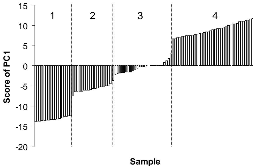
FIG. 2- Scores of the first principal component of the Pong Su samples in ascending order. Four groups are identified.
