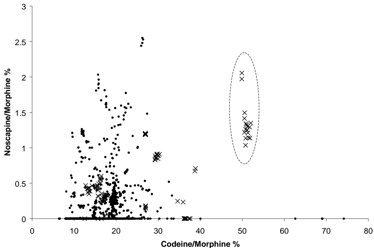
FIG. 3- Data of figure 1 (crosses) with 1533 samples of authentic Southeast Asian heroin seized in Australia during 2002- 2003 (closed circles). The group within the dashed oval is that identified as "1" in the PC plot of Figure 2.
