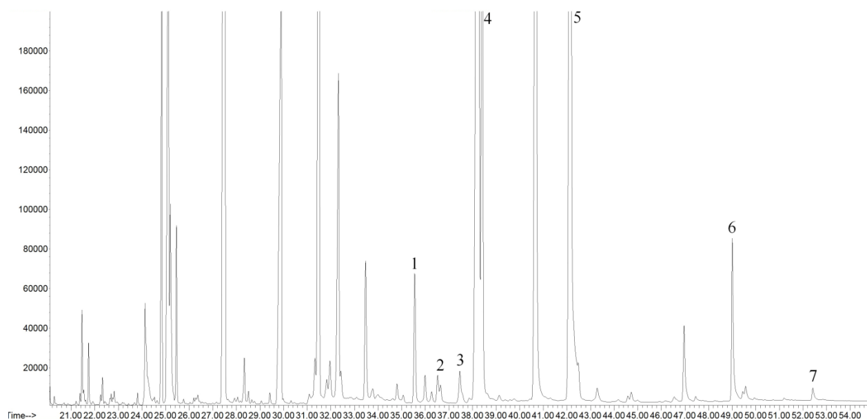
FIG. 4- Total ion current chromatogram of the acid/neutral extract of a heroin sample seized from the Pong Su. 1: O6,N-diacetylnorcodeine; 2: O6,N-
