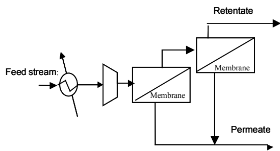
Figure 2 A two-stage series membrane system configuration (TSMS)
