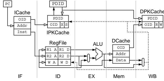
Fig. 2. Example Legba pipeline.
