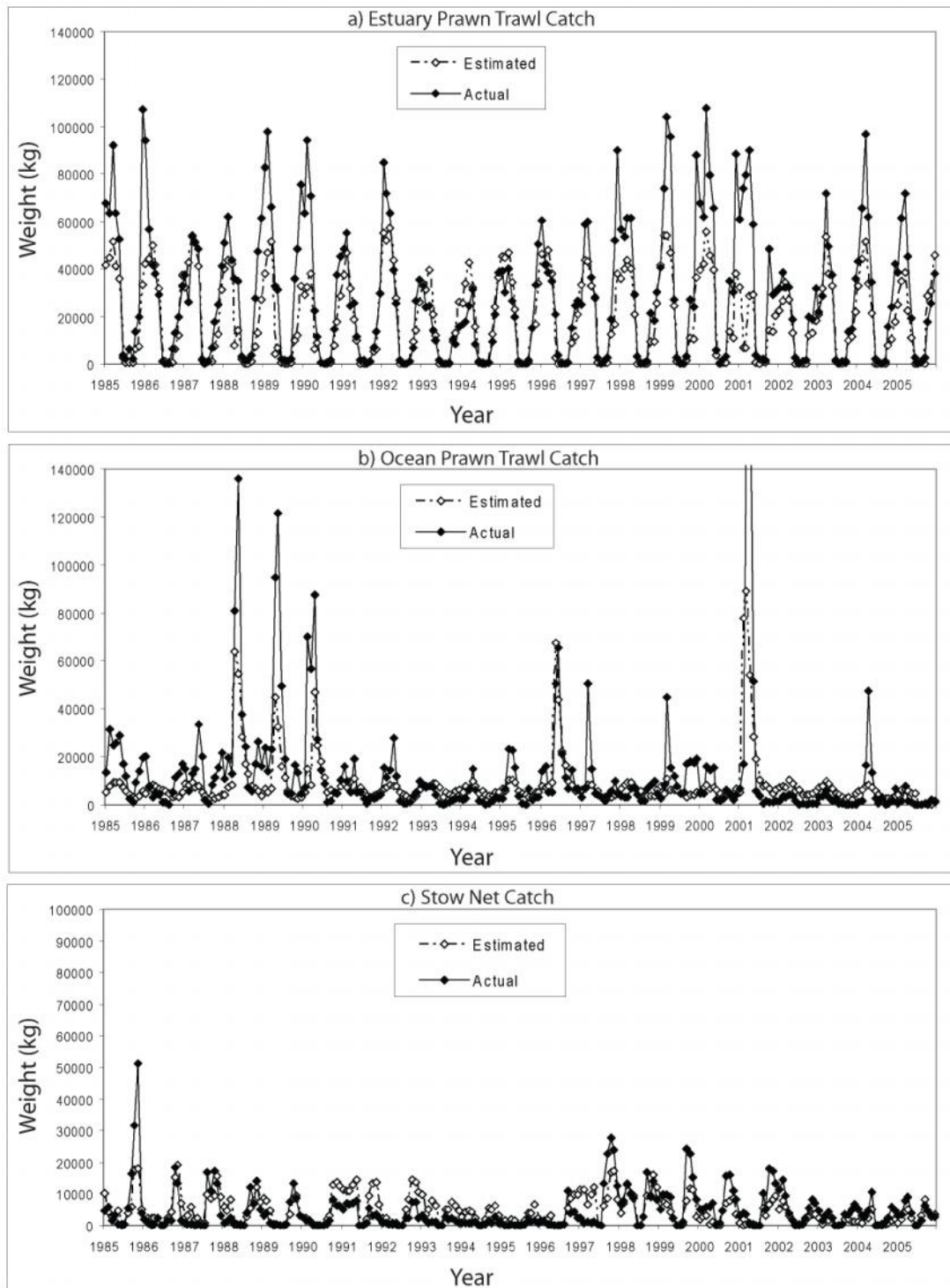
Figure 4: Modelled and observed catches from the three fishing methods considered in the present study from the Clarence River and Ocean Zone 2 (29° and 30°S) from January 1985 to December 2005. (a) Estuary Prawn Trawl; (b) Ocean Prawn Trawl; (c) stow netting.
