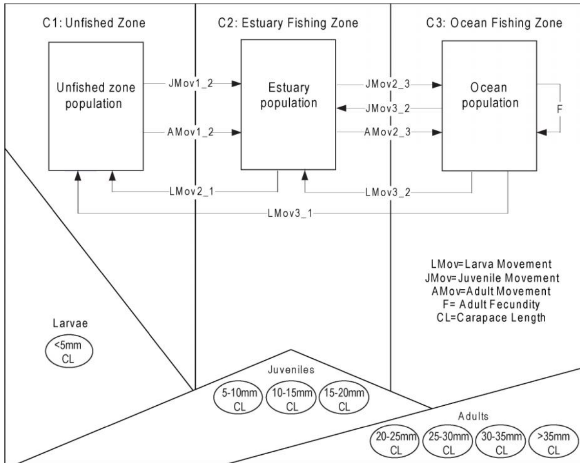
Figure 2: The stage-size structured metapopulation model showing the three model compartments (C1–C3). The upper area displays the three metapopulation stocks within each compartment and shows the movement between the populations. The lower area displays the various life stages based on carapace lengths (CL) into which individuals are graded. The polygons provide a stylistic representation of the relative numbers of individuals of the three main life stages – larva, juvenile and adult – and in which compartment these life stages predominantly reside.
