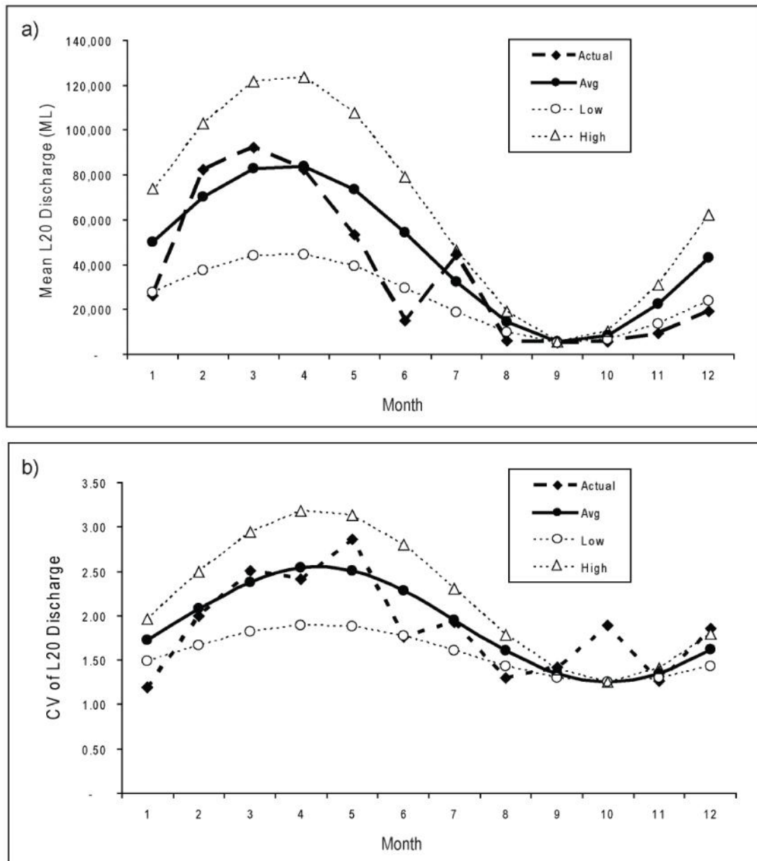
Figure 3: Sine curves used to model seasonal variation in the (a) mean and (b) coefficient of variation (CV) of log-normal distributions fitted to historical maximum river discharge data. The Actual line shows the values from the historical record and the Low, Avg and High lines show the values used in their respective scenarios.
