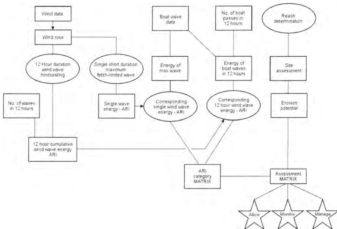
Figure C-1: Flow Diagram of the Decision Support System
