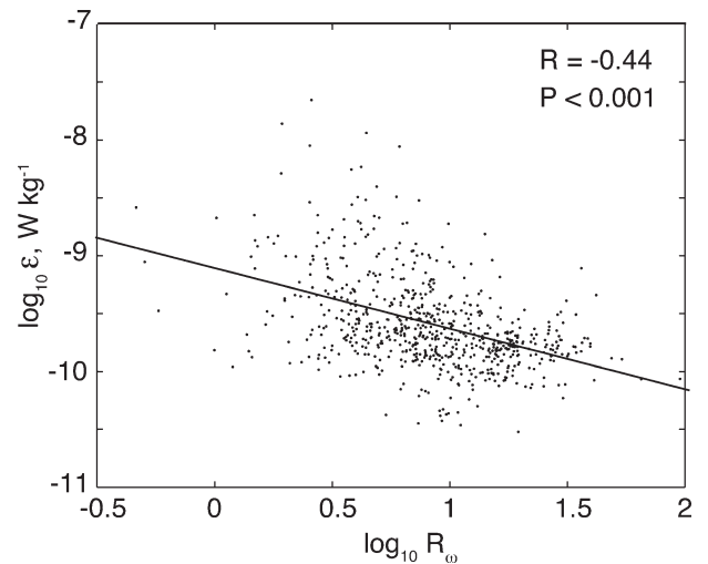
Figure 9. Correlation between the shear-to-strain variance ratio, R_\omega , and microstructure-deduced dissipation rates, \epsilon_{\text{micro}} , for all data. The correlation coefficient, R and p value, P , are indicated.
