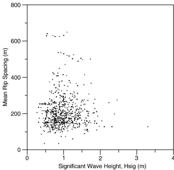
Fig. 8. Mean rip spacing (MRS) vs. significant wave height.
