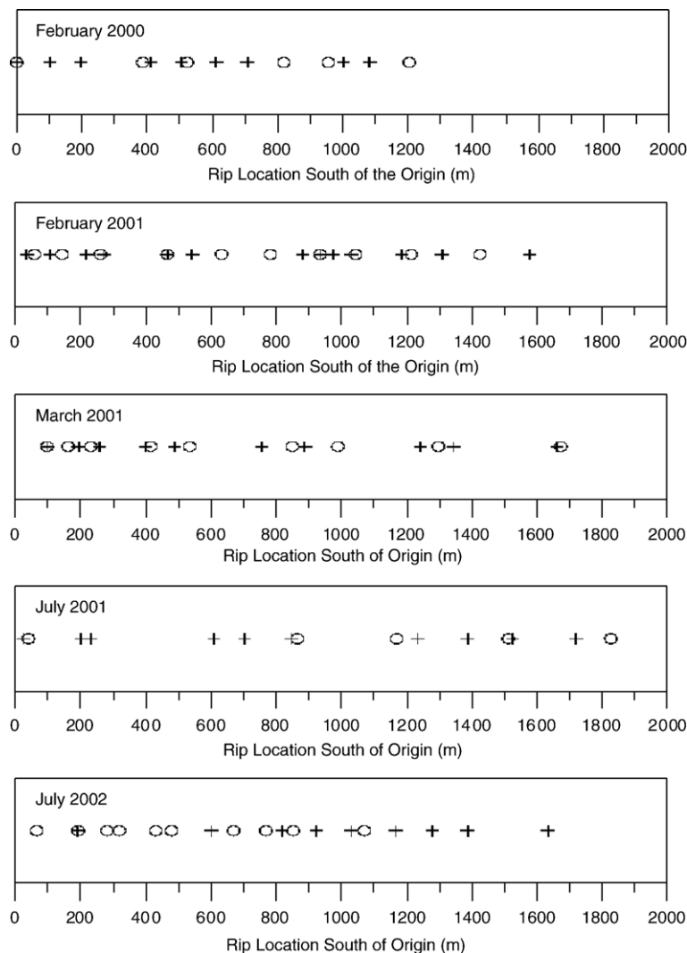
Fig. 5. Rip locations before and after 5 example 'system reset' events. (+ denotes pre-storm locations, o denotes post-storm locations).
