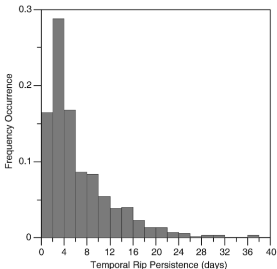
Fig. 9. Frequency histogram of temporal rip persistence.
