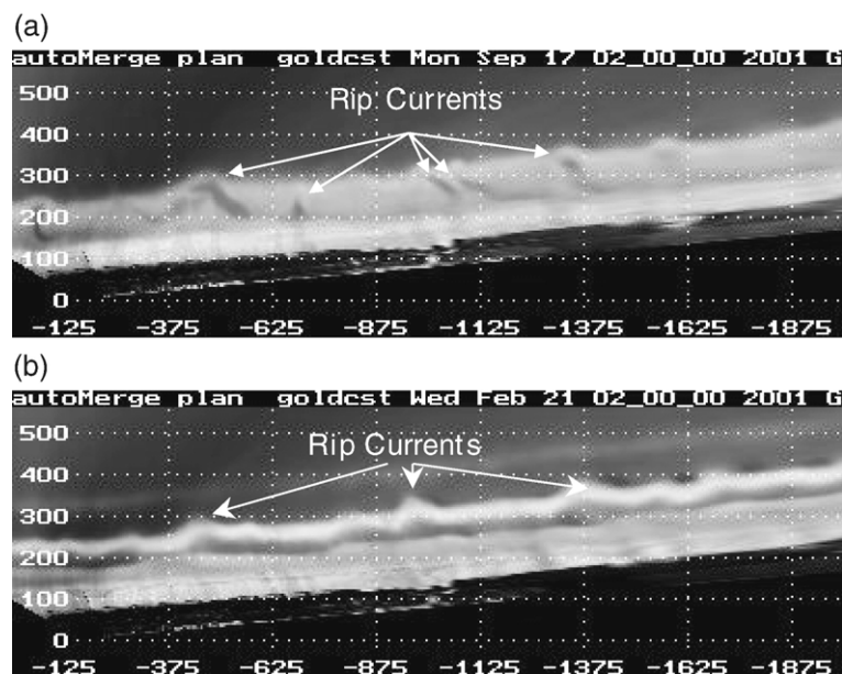
Fig. 2. Rectified daytimex image of the 2 km study area with rips identified by two image ‘signatures’: (upper panel) alternating transverse channel/bar morphology, and (lower panel) crescentic features in the longshore sand bar.
