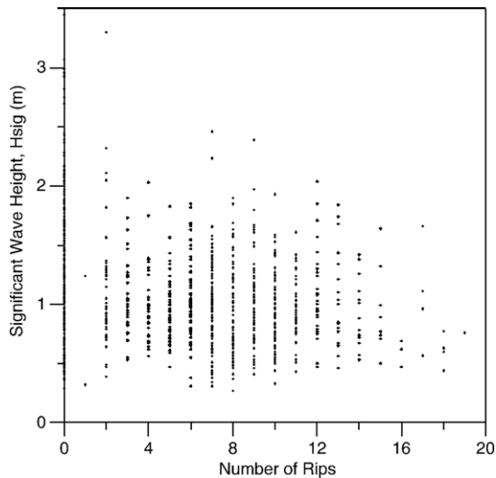
Fig. 6. Number of observed rips within the 2 km study area vs. significant wave height.
