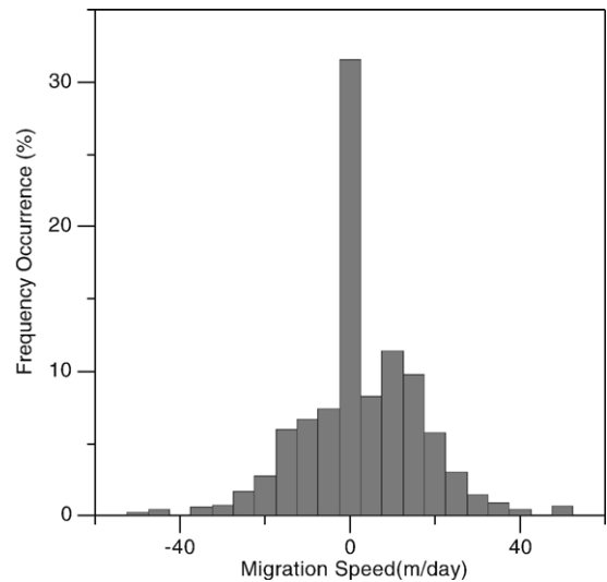
Fig. 10. Frequency histogram of all migration events observed over the three year study period.
