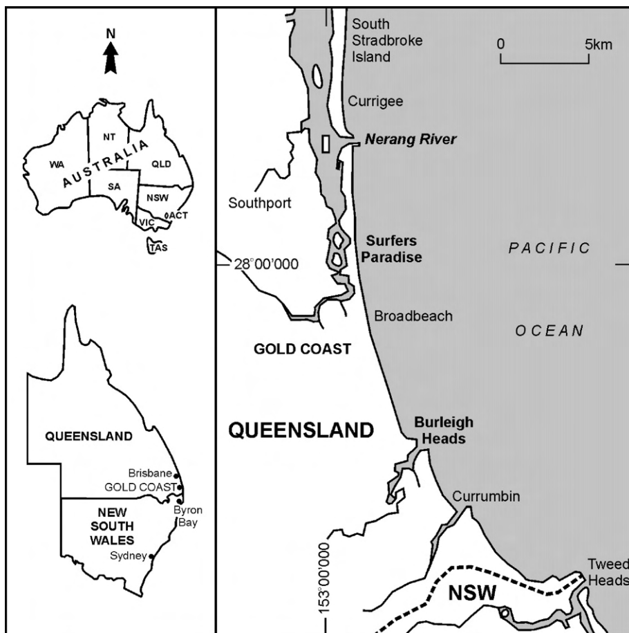
Fig. 1. Northern Gold Coast study site.
