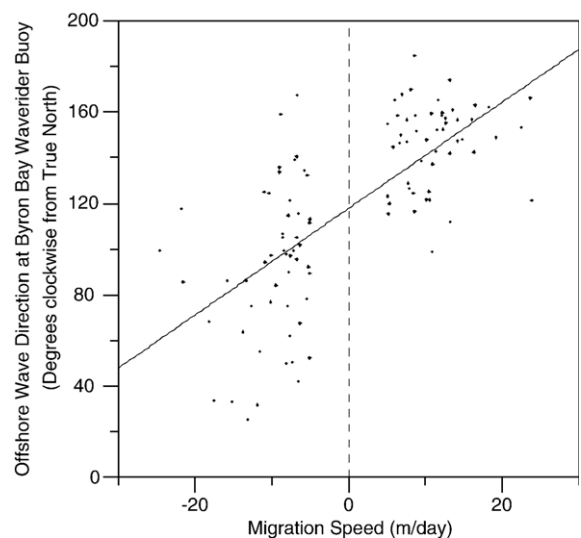
Fig. 11. Average daily rip migration vs. offshore wave direction for the special cases of H_s < 1.5 m, T_p < 10 s and observed migration speeds greater than 5 m/day.
