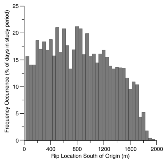
Fig. 4. Frequency histogram of rip location (50 m alongshore bins) within 2 km study area, for the three year study period.
