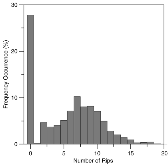
Fig. 3. Frequency histogram of number of rips per day within 2 km study area, for the three year study period.
