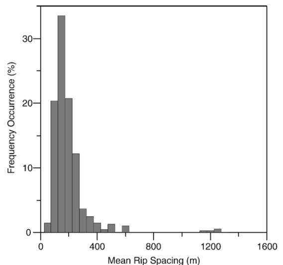
Fig. 7. Frequency histogram of mean rip spacing (MRS).
