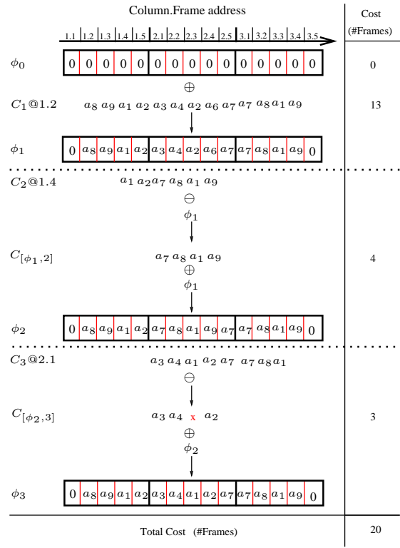
Figure 1. A motivational example.
