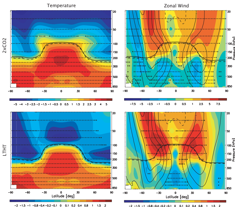
Fig. 7. 2\times\text{CO}_2 (top) and LTHT (bottom) annual mean temperature (left) and zonal wind (right) response. LTHT results, and significance symbols, are as in Fig. 3. Note contour differences between 2\times\text{CO}_2 and LTHT.
