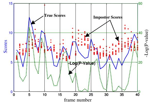
Figure 1. Frame-based scores from speaker and impostor models and its corresponding frame-based P -value for first forty frames of a male target test speech segment from the NIST 2002 Dataset
