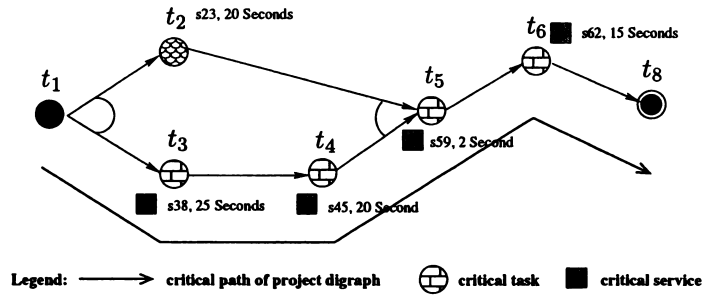
Figure 4.3: Critical Path
