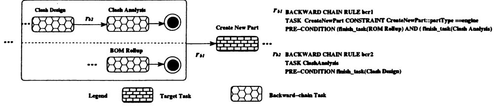
Figure 3.11: Backward-chain Inference
