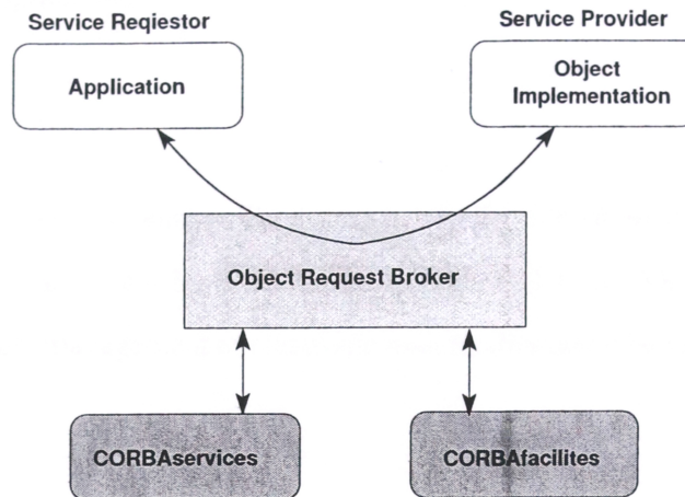
Figure 2.4: CORBA architecture
