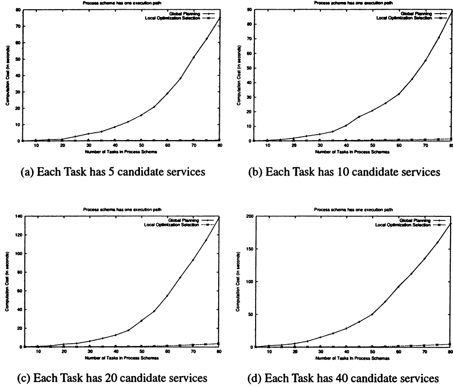
Figure 6.9: Experimental Results (computation cost) in a Dynamic Environment, Varying the Number of Tasks in Process Schema and the Number of Candidate Services for Each Task.
