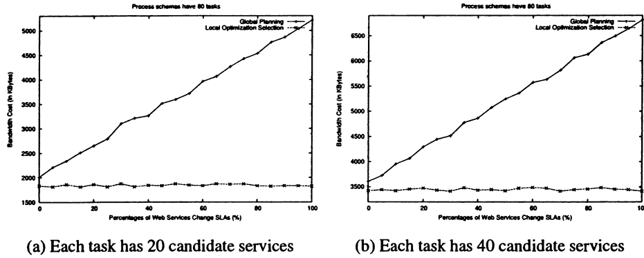
Figure 6.12: Experimental Results (bandwidth cost) in a Static Environment, Varying the Percentage Services Change SLAs and the Number of Candidate Services for Each Task.
