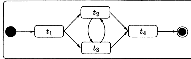
Figure 4.4: "Unfoldable" Statechart
