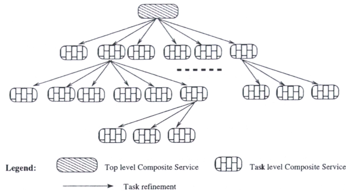
Figure 3.5: Composition Hierarchy
