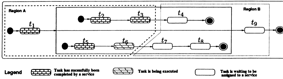
Figure 5.1: Partition a Composite Service into Regions for Regenerating Process Schema
