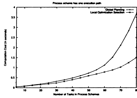
(b) Each Task has 10 candidate component services
