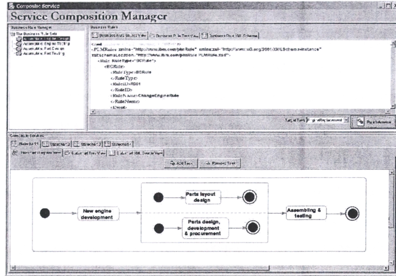
Figure 6.3: GUI of Service Composition Manager
