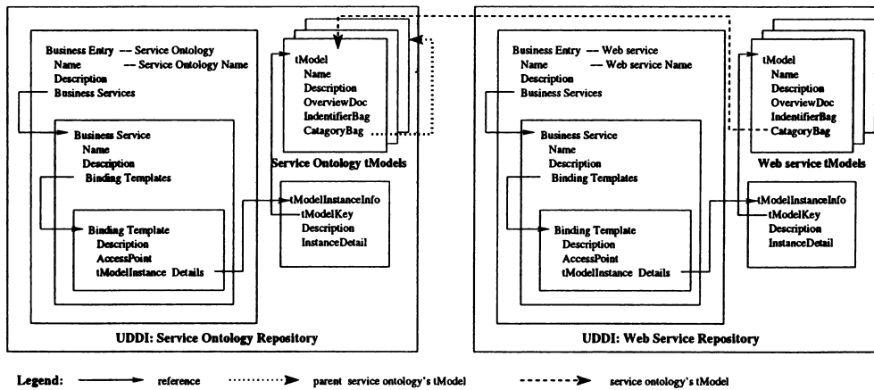
Figure 6.2: Service Ontology Repository and Web Service Repository
