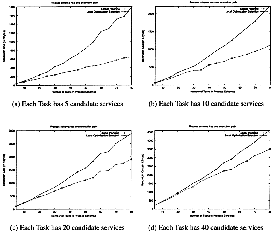
Figure 6.11: Experimental Results (bandwidth cost) in a Dynamic Environment, Varying the Number of Tasks in Process Schemas and the Number of Candidate Services for Each Task.
