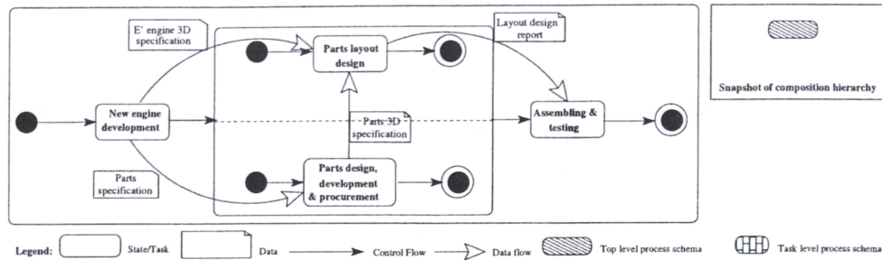
Figure 3.7: Top Level Process Schema for Replacing Engine
