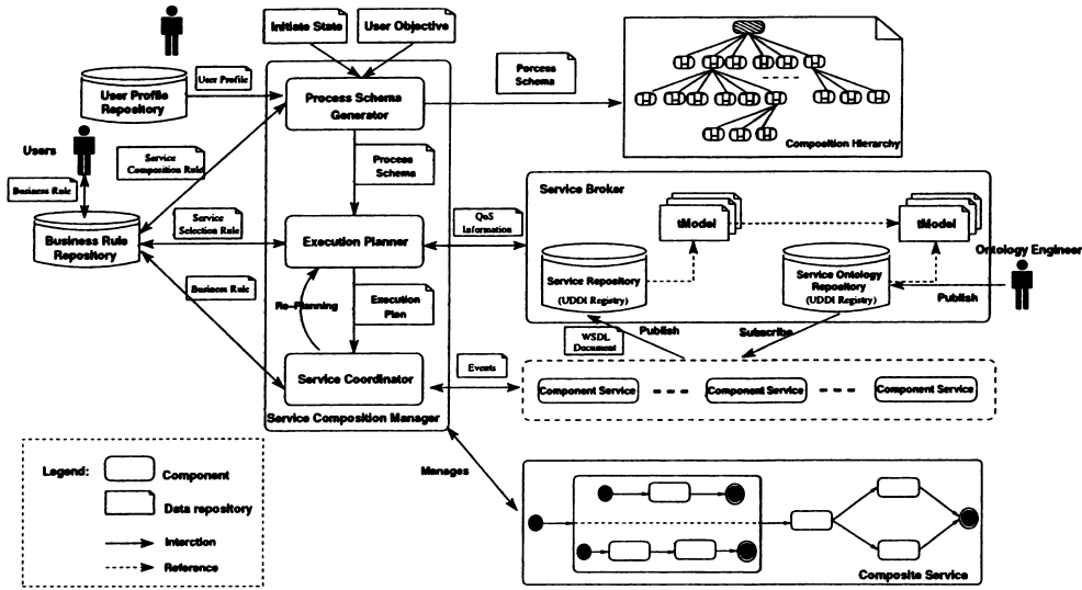
Figure 6.1: Architecture of the DY_{flow} Prototype
