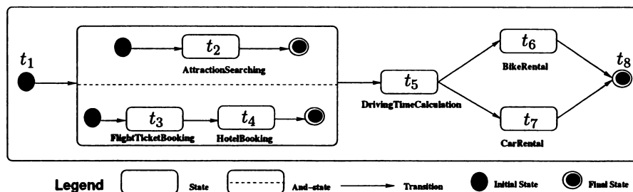
Figure 4.1: Statechart of a Composite Service “Travel Planner”
