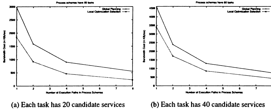
Figure 6.13: Experimental Results (bandwidth cost) in a Static Environment, Varying the Number of Execution Paths in Process Schemas and the Number of Candidate Services for Each Task.
