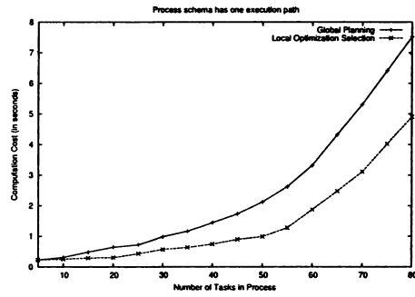
(d) Each Task has 40 candidate component services
