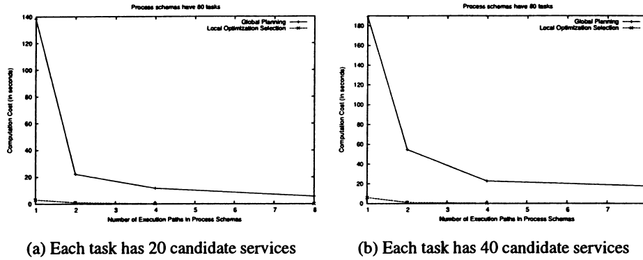
Figure 6.10: Experimental Results (computation cost) in Dynamic Environment, Varying the Number of Execution Paths in Process Schemas and the Number of Candidate Services for Each Task.
