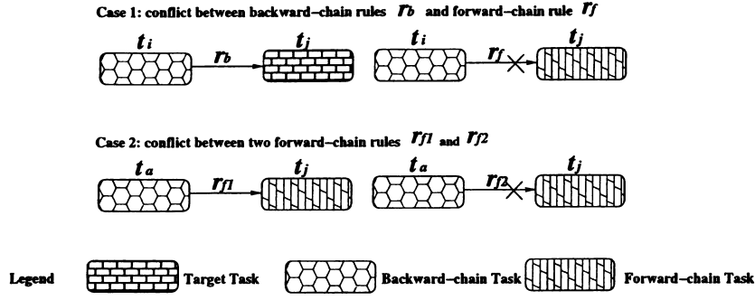
Figure 3.14: Conflict Between the Rules
