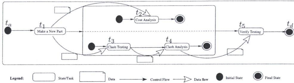
Figure 3.3: Defining Process Schema Using a Statechart
