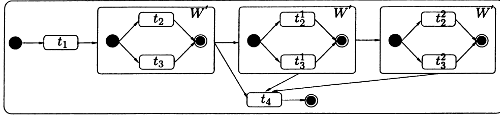
Figure 4.6: Acyclic Statechart Derived from That in Figure 6.
