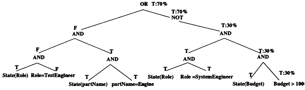
Figure 3.13: Annotated Condition Tree
