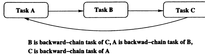
Figure 3.10: Cyclic Graph
