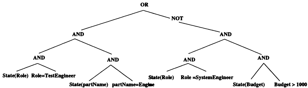
Figure 3.12: Condition Tree
