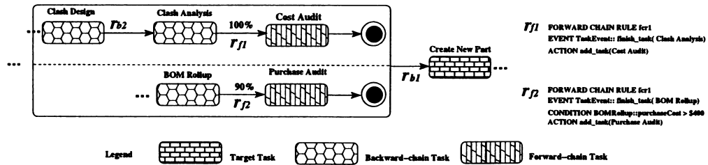
Figure 3.15: Forward-chain Inference
