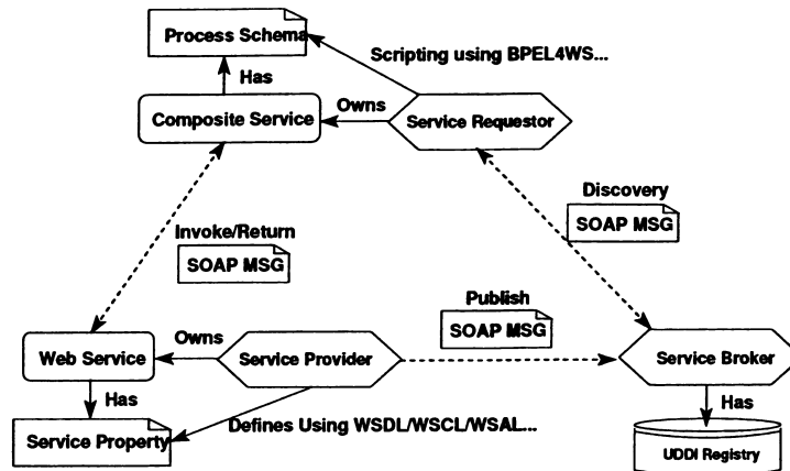
Figure 2.5: Web Service Architecture
