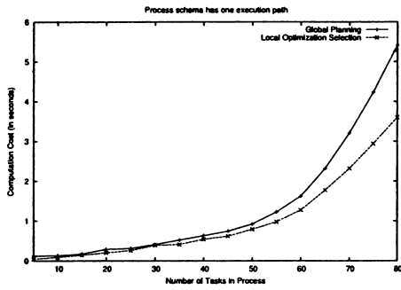
(c) Each Task has 20 candidate component services
