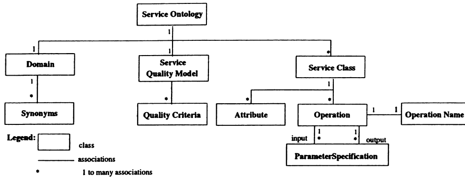
Figure 3.2: UML Class Diagram for Service Ontology
