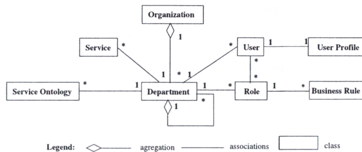
Figure 3.4: UML Class Diagram for Organizational Structure
