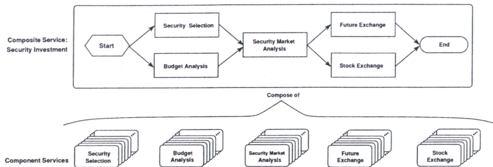
Figure 2.2: Service Composition: A Running Example
