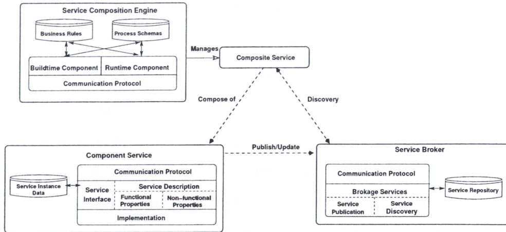
Figure 2.3: Architecture of Service Composition Framework
