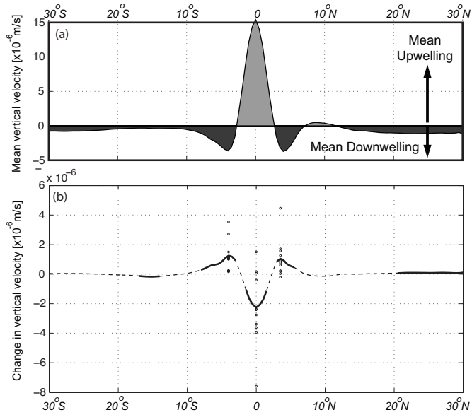
Fig. 7 a) Vertical velocities of water ( 10^{-6} \text{ m.s}^{-1} ) at a depth of 50 m, for 1990 (mean 1980 – 1999), averaged between 170°E and 110°W, where a positive velocity corresponds to upwelling and a negative velocity to downwelling; and b) Climate driven changes to vertical velocities for 2100 (full line if significant at 95%; dashed line otherwise). Values for individual CMIP3 models are indicated in the maxima (small circles). The strong equatorial upwelling shows decreases that are immediately balanced by strong downwelling near 4°N–4°S so that net upwelling between 9°S and 9°N does not change.
