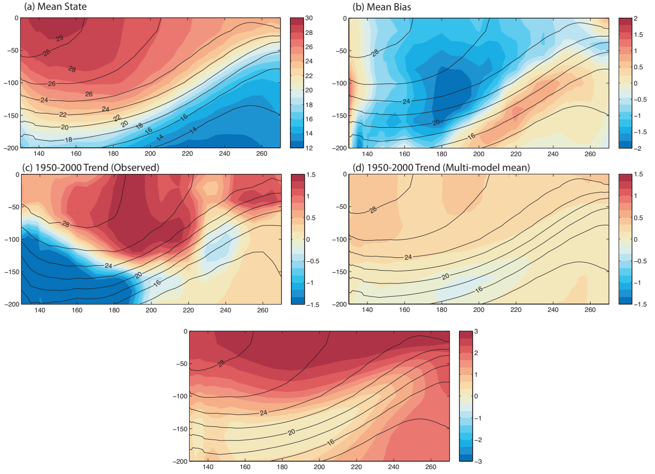
Fig. 3 Equatorial potential temperature averaged 5^{\circ}\text{S} to 5^{\circ}\text{N} ( ^{\circ}\text{C} ) as a function of longitude and depth. a) Observed long-term mean b) Model bias (MMM – observations). c) Observed linear temperature trend over 50 years. d) MMM trend over 1950-2000. e) Projected trend in temperatures 2000-2100 (color shading). Overlaid (line contours) is the MMM 1950-2000 mean (a,b,d,e) and observed long-term mean (c). Observations are based on a new dataset (Durack and Wijffels 2010; Johnson and Wijffels 2011) that has used observations from 1950-2008 to compute the mean state and trends (expressed as a 1950-2000 trend). Multi-parametric regression technique was employed to reduce aliasing of the trend by various modes of climate variability including ENSO and the PDO.
