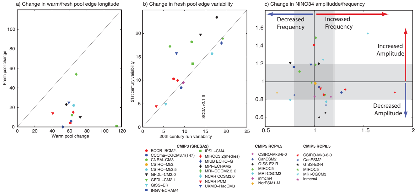
Fig. 2 Changes in WP and ENSO variability. a) change in the longitude of the equatorial ( 3^{\circ}\text{S} to 3^{\circ}\text{N} ) warm pool and fresh pool edge over the 21st century in individual CMIP3 models. b) change in the variability of the fresh pool edge ( ^{\circ}\text{longitude} , 1 standard deviation). The fresh pool and warm pool are defined by model specific isohalines and isotherms, respectively, chosen such that the area of bounded freshwater or warm water was equivalent to the area contained within the T = 29^{\circ}\text{C} isotherm and S = 34.8 isohalines in the observations from CARS. c) Ratio of 2050-2100 to 1950-2000 frequency and amplitude of temperature anomalies (NINO3.4 index). Amplitude corresponds to one standard deviation. Frequency was computed as a weighted average of NINO3.4 frequency by spectral power for all frequencies whose power was significant at 95% level. Panels (b) and (c) contain addition preliminary results from the CMIP5 archive. CMIP5 data is still in progress and modelling groups may replace certain data in the future. The shaded area delimits the 20% change.
